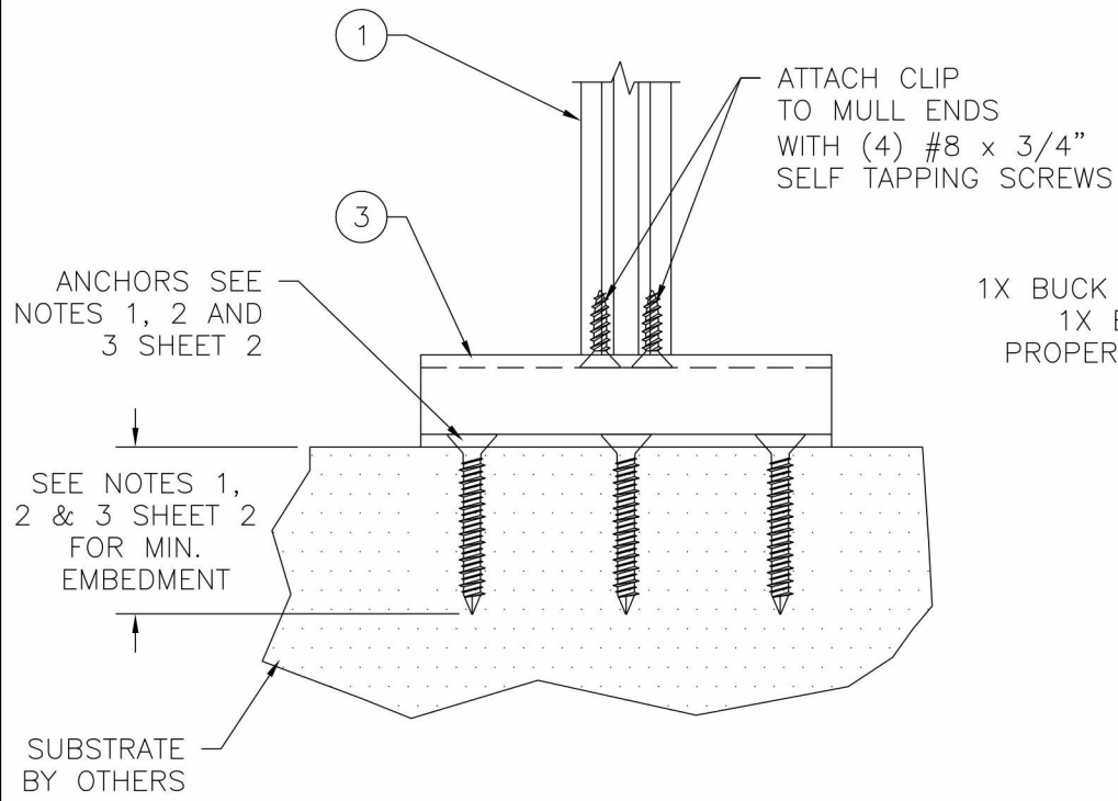
ALTERNATE MULL CLIP 10300093 INSTALLATION DETAILS SILL, SHOWN, HEAD AND JAMBS SIMILAR.
