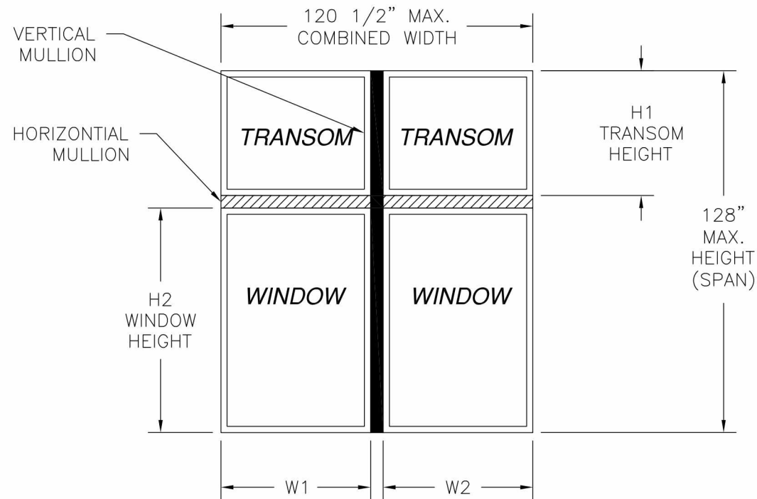
10300085 ALUMINUM X MULLION NON REINFORCED LMI WIND ZONE 3
