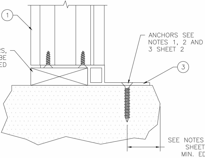
ALTERNATE MULL CLIP 10300093 INSTALLATION DETAILS SILL, SHOWN, HEAD AND JAMBS SIMILAR.
