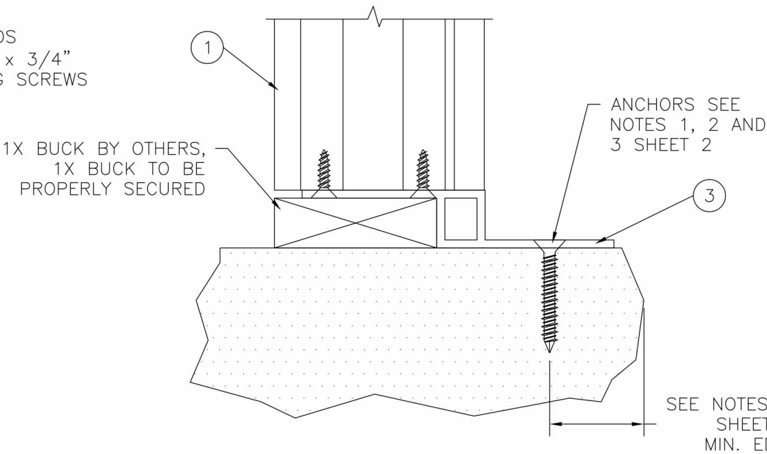
ALTERNATE MULL CLIP 10300093 INSTALLATION DETAILS SILL, SHOWN, HEAD AND JAMBS SIMILAR.
