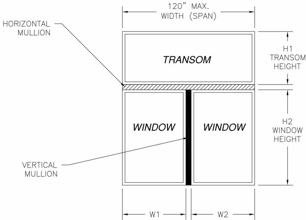
10300085 ALUMINUM T MULLION NON REINFORCED LMI WIND ZONE 3
