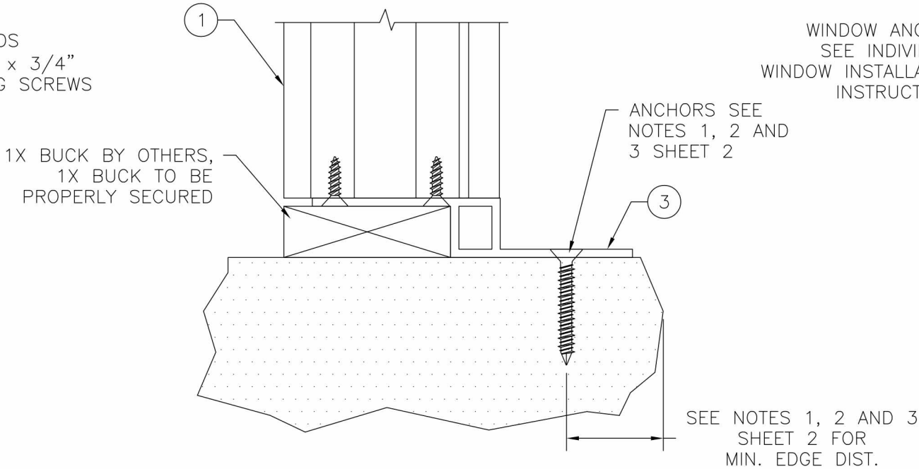
ALTERNATE MULL CLIP 10300093 INSTALLATION DETAILS SILL SHOWN, HEAD SIMILAR.
