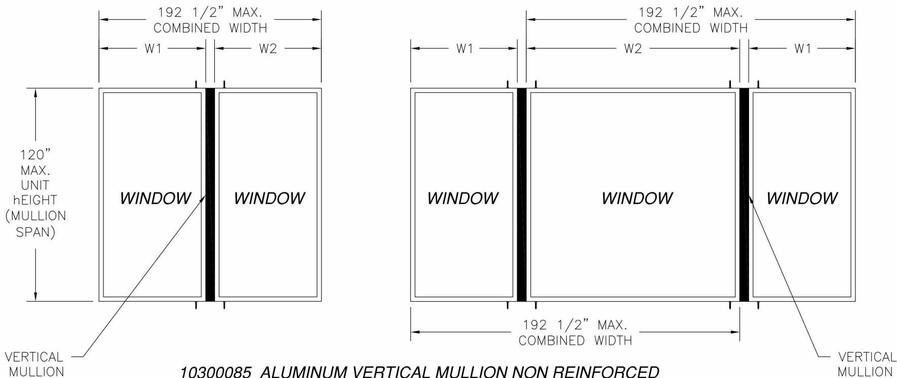
10300085 ALUMINUM VERTICAL MULLION NON REINFORCED LMI WIND ZONE 3
