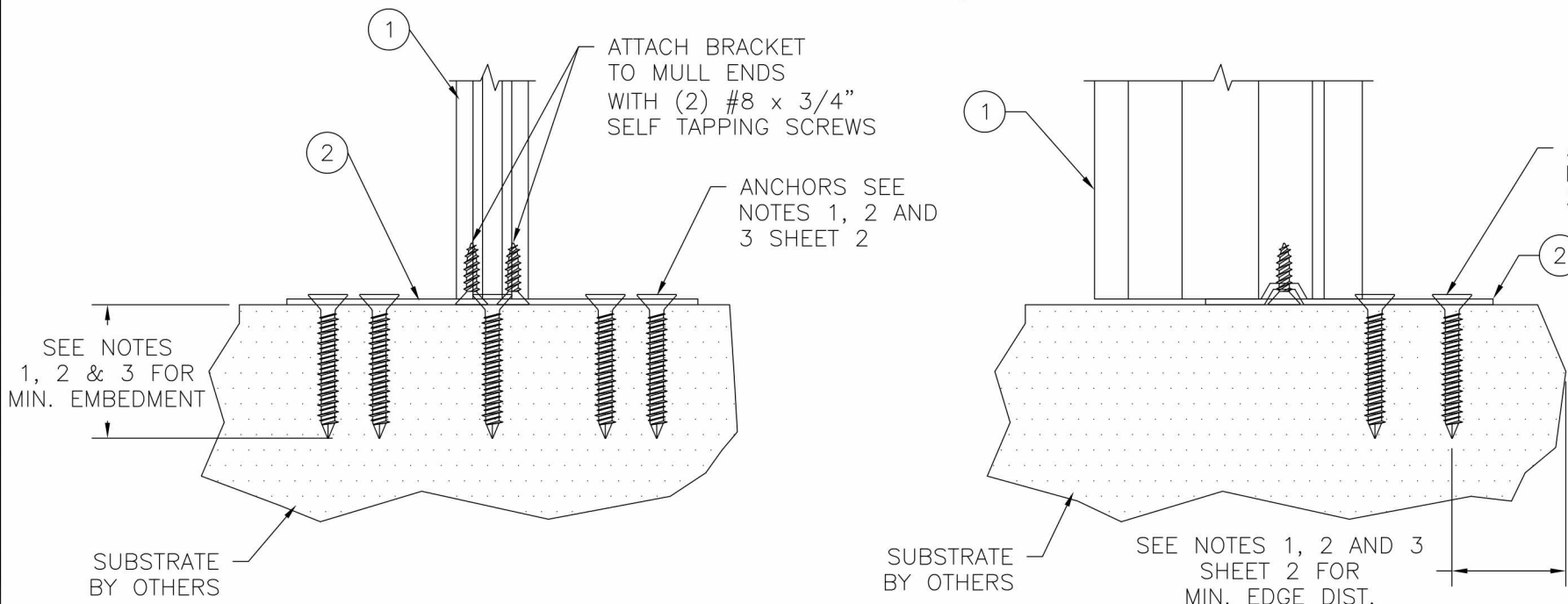
STEEL MULION BRACKET 10203000 INSTALLATION DETAILS SILL SHOWN, HEAD SIMILAR.
