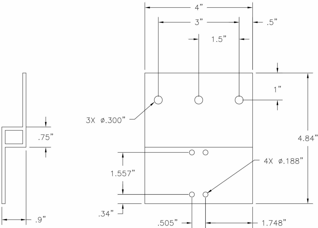
3 MULL CLIP ALUMINUM 6005-T5 .125" THICK
