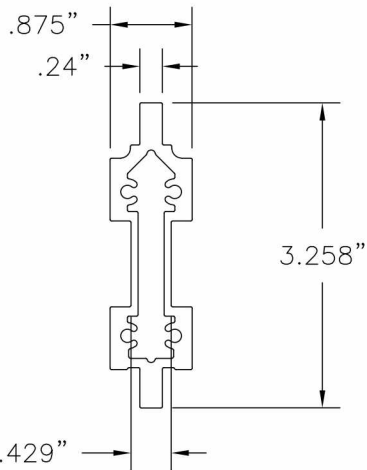
1 10300085 ALUMINUM VERTICAL MULLION ALUMINUM 6005-T5 .075" THICK MINIMUM
