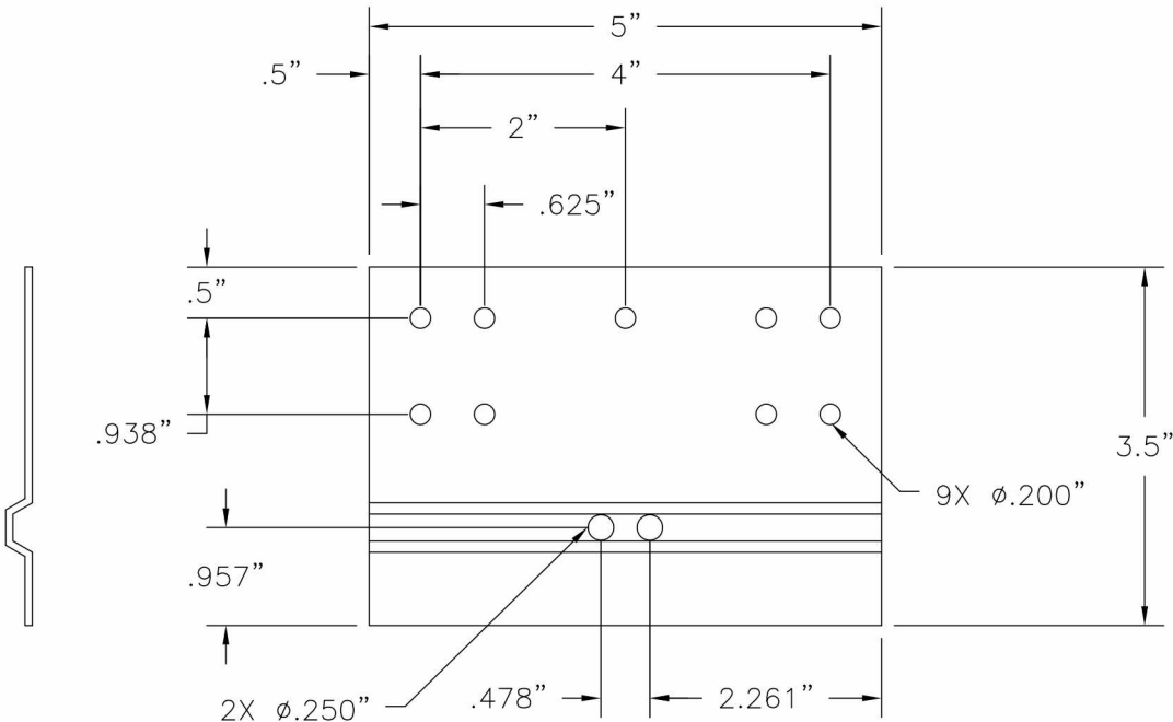
2 STEEL MULLION BRACKET 15GA. GALVANIZED STEEL
