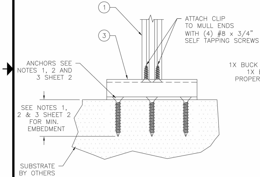
ALTERNATE MULL CLIP 10300093 INSTALLATION DETAILS SILL SHOWN, HEAD SIMILAR.
