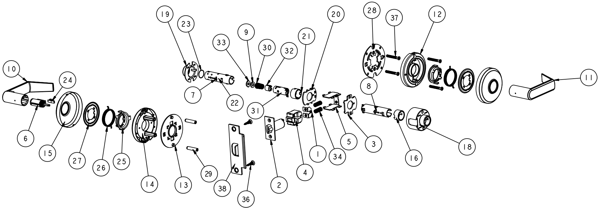
QCL 270 1/2" MIN. LATCH THROW (STEEL)
