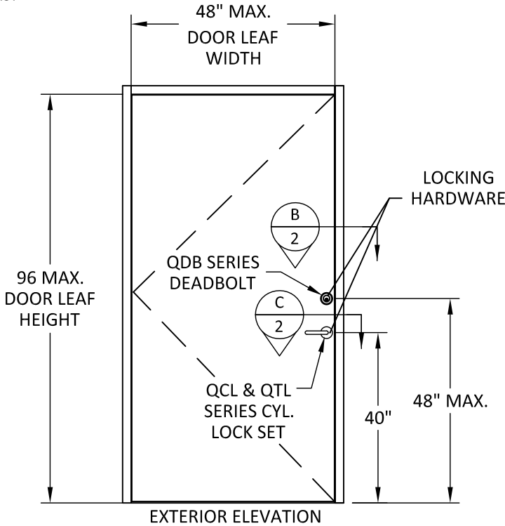
SINGLE STEEL DOOR DOORS UNDER SEPARATE APPROVAL
