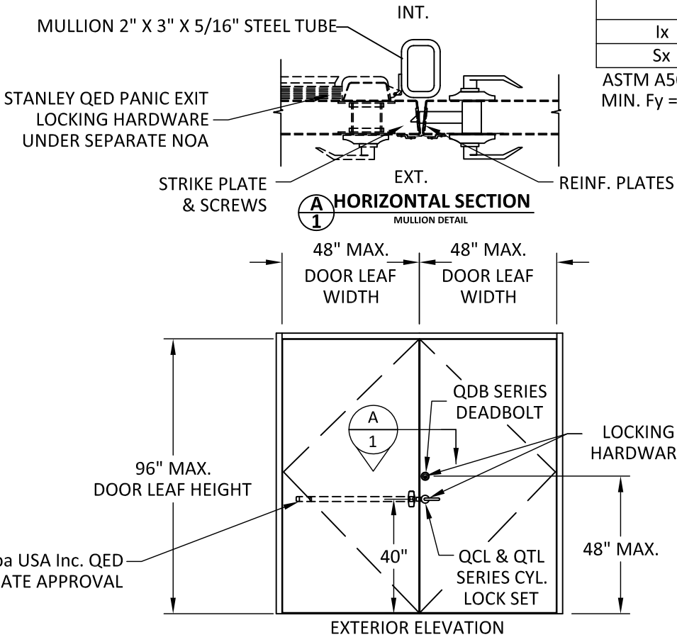
TWO SINGLE STEEL DOORS WITH INTERMEDIATE MULLION DOORS & MULLION UNDER SEPARATE APPROVAL
