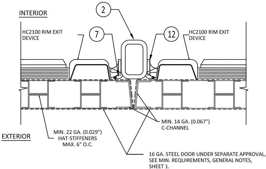
B HORIZONTAL SECTION 3 HC2100 RIM EXIT W/ HCK822 MULLION DOUBLE DOOR APPLICATION
