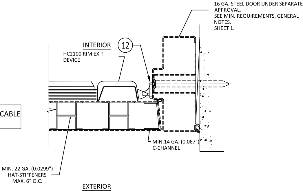
A HORIZONTAL SECTION 3 HC2100 RIM EXIT SINGLE DOOR APPLICATION
