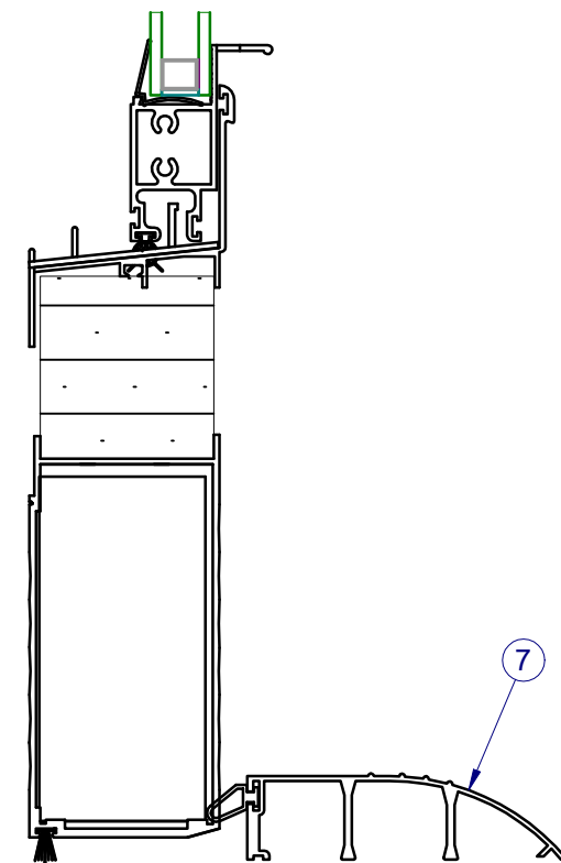
ALT. THRESHOLD (1126)
