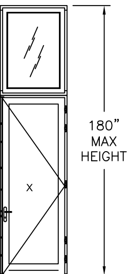
SINGLE DOOR WITH FIXED WINDOW
