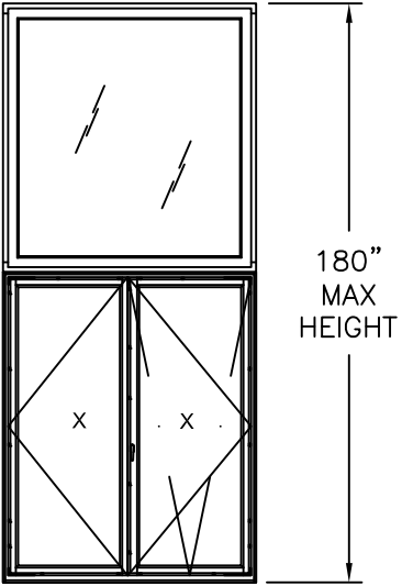
DOUBLE CASEMENT WITH FIXED WINDOW
