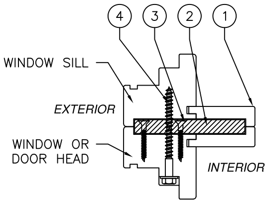
MULLION CROSS SECTION
