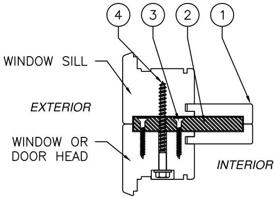
MULLION CROSS SECTION
