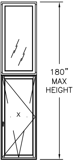
SINGLE CASEMENT WITH FIXED WINDOW
