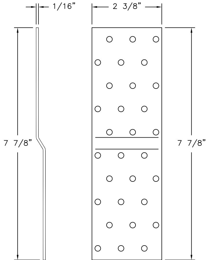
⑤ CLIP 14 GA GALVANIZED STEEL
