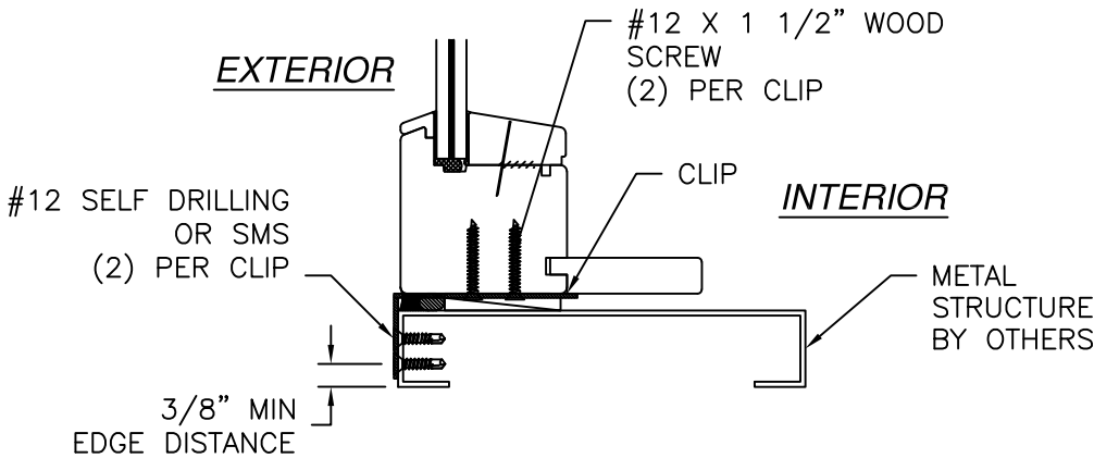
FLUSH INSTALLATION METAL STRUCTURE INSTALLATION SILL SHOWN HEAD AND JAMB SIMILAR
