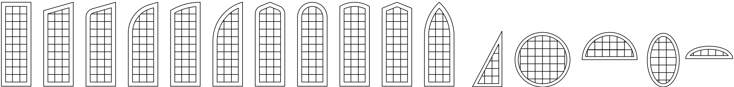
WINDOW UNITS WITH SDL
