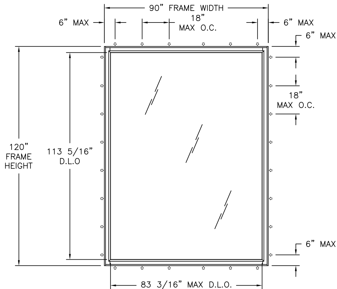
PICTURE WINDOW - DIRECT SET EXTERIOR VIEW
