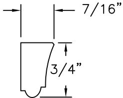
⑧ GLASS STOP WOOD SPECIFIC GRAVITY G.59 MIN
