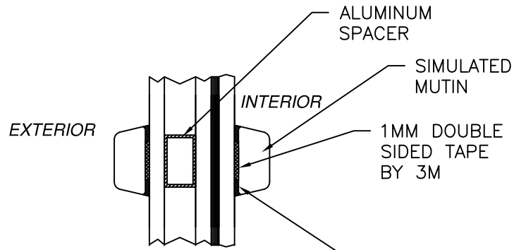
SIMULATED DIVIDED LITE (SDL) CROSS SECTION
