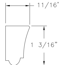
⑬ GLASS STOP WOOD SPECIFIC GRAVITY G.59 MIN
