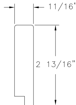
⑥ JAMB EXTENSION WOOD SPECIFIC GRAVITY G.59 MIN
