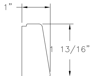
④ GLASS STOP WOOD SPECIFIC GRAVITY G.59 MIN
