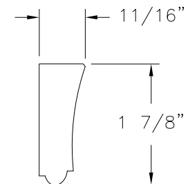
⑫ GLASS STOP WOOD SPECIFIC GRAVITY G.59 MIN
