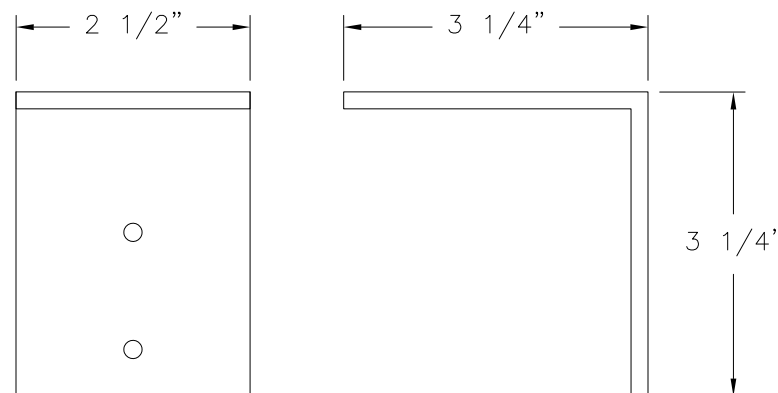
⑮ CLIP (HL33) 7 GA GALVANIZED STEEL
