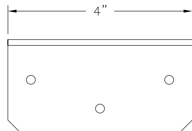
⑭ CLIP (M24) 12GA GALVANIZED STEEL
