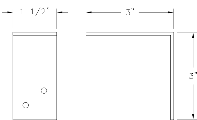
② CLIP (A33) 12 GA GALVANIZED STEEL
