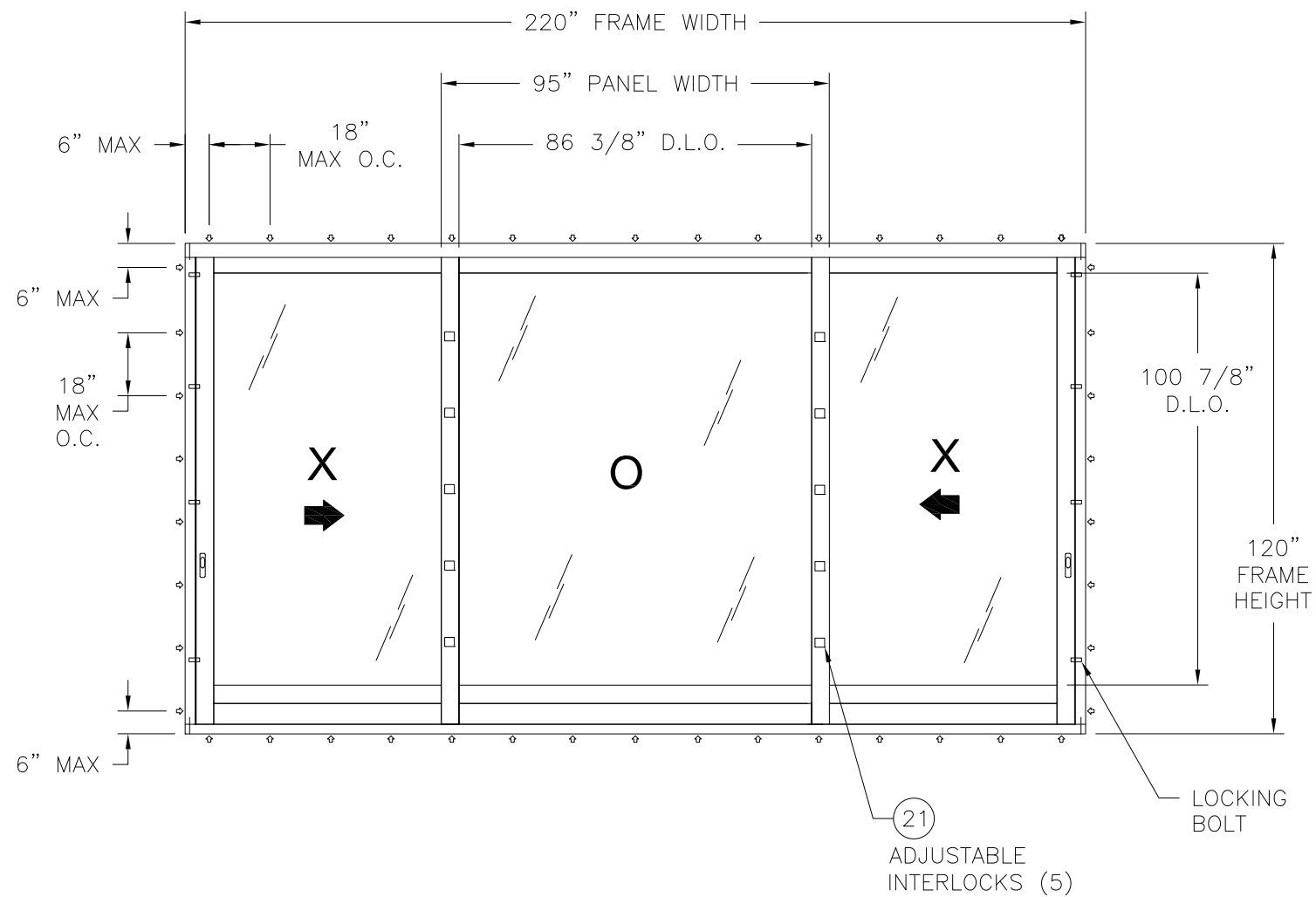
LIFT & SLIDE ALUMINUM CLAD DOOR INTERIOR VIEW
