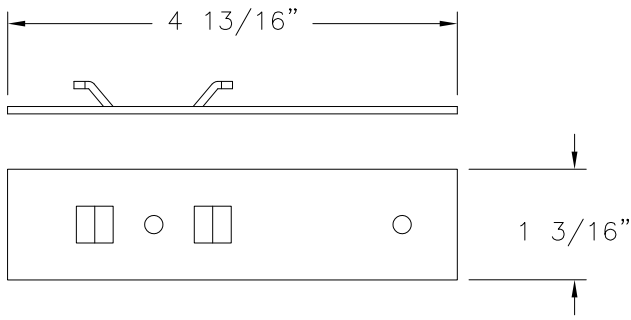
36 SHIM THERMOSTEP GALVANIZED STEEL .080 THICK
