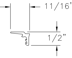
32 WEATHERSTRIP EPDM 75 SHORE A
