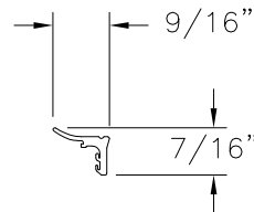
31 WEATHERSTRIP EPDM 75 SHORE A
