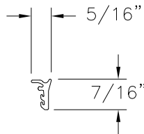
30 WEATHERSTRIP EPDM 75 SHORE A
