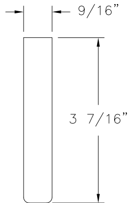
④ FRAME WOOD SPECIFIC GRAVITY G.45 MIN
