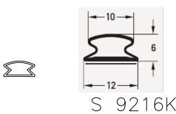
33 SELF-ADHESIVE GASKET SILICONE
