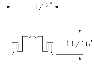
27 GUIDE PROFILE ALUMINUM 6063-T5
