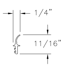
29 WEATHERSTRIP EPDM 75 SHORE A
