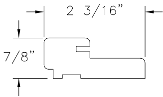
⑮ INTERLOCK ASTRAGAL WOOD SPECIFIC GRAVITY G.45 MIN
