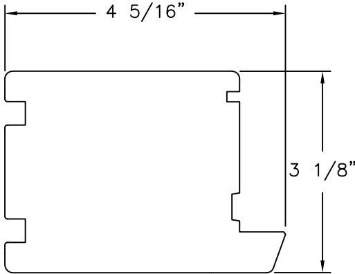
⑧ SASH WOOD SPECIFIC GRAVITY G=0.59 MIN.
