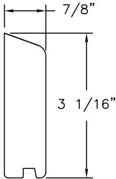
⑫ DRIP BATTEN WOOD SPECIFIC GRAVITY G=0.59 MIN.
