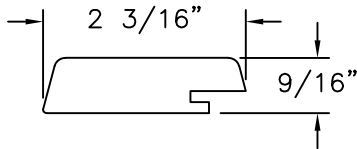
⑭ ASTRAGAL WOOD SPECIFIC GRAVITY G=0.59 MIN.
