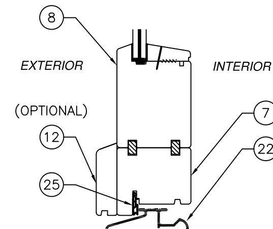
VERTICAL CROSS SECTION HORIZONTAL RAIL OPTIONAL SEE NOTE 13 SHEET 1
