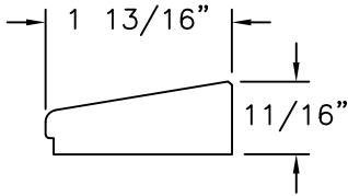
⑨ GLASS STOP WOOD SPECIFIC GRAVITY G=0.59 MIN.
