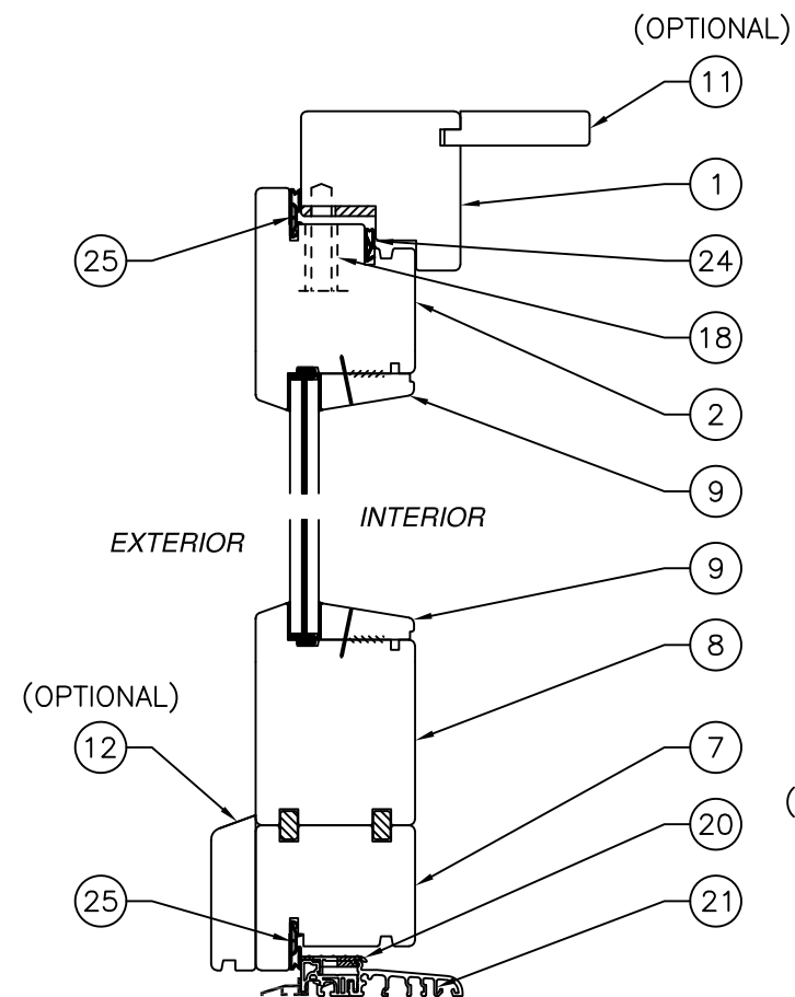
VERTICAL SECTION
