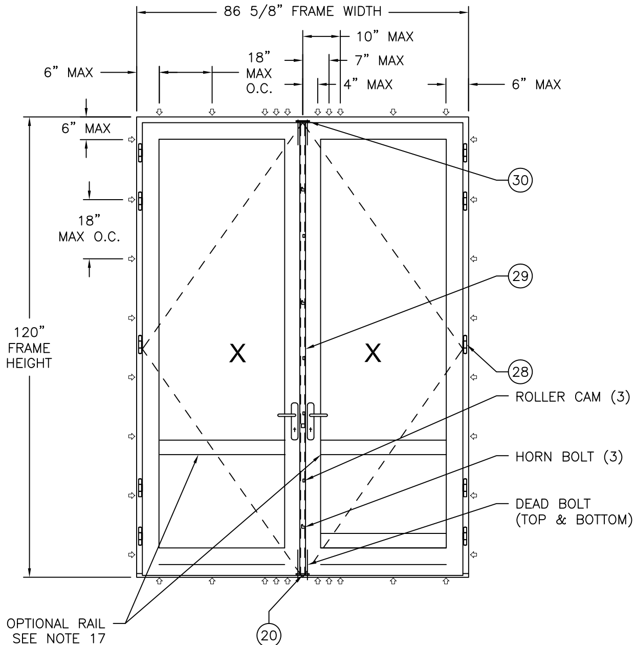
OUTSWING DOOR - DOUBLE EXTERIOR VIEW
