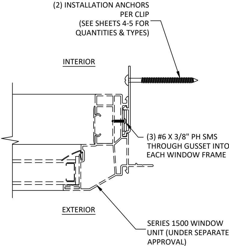
ANCHOR CLIP DETAIL SIDE VIEW
