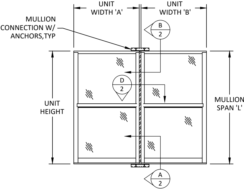
ONE-WAY MULLION EXAMPLE
