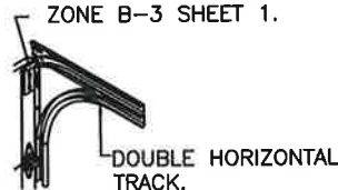
DOUBLE TRACK LOW HEADROOM OPTION (AVAIL. FOR BOTH 2" AND 3" TRACK)
