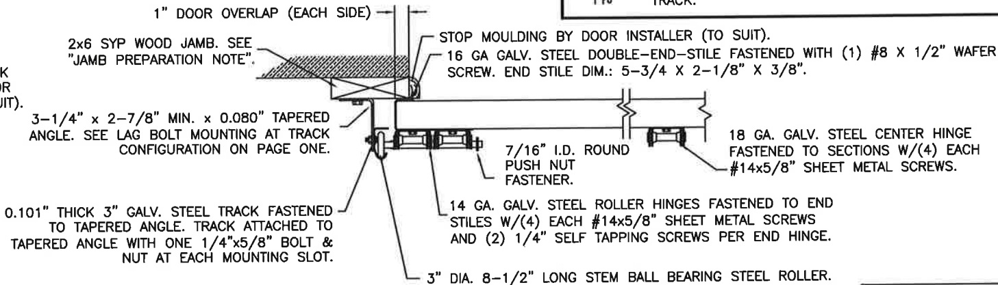
SECTION C-C
