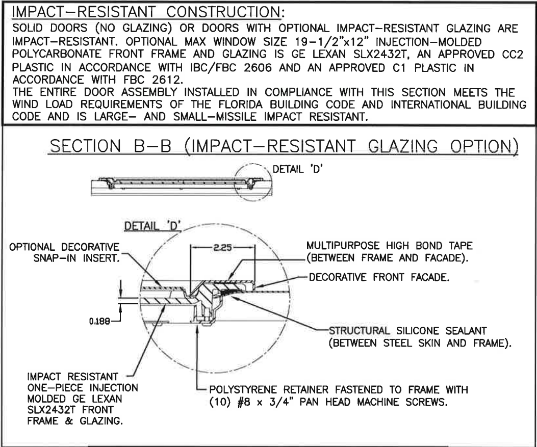
IMPACT-RESISTANT ASSEMBLY DETAILS DRAWING 104751-A
