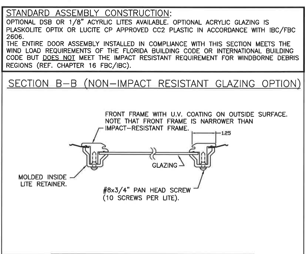
STANDARD ASSEMBLY DETAILS DRAWING 104751-B
