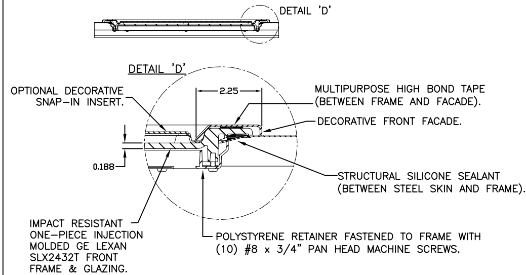
IMPACT-RESISTANT ASSEMBLY DETAILS DRAWING 104724-A
