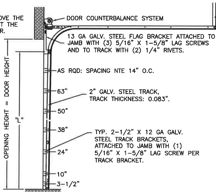
2" TRACK CONFIGURATION DOORS UP TO 800 LBS.
