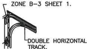
DOUBLE TRACK LOW HEADROOM OPTION (AVAIL. FOR BOTH 2" AND 3" TRACK)
