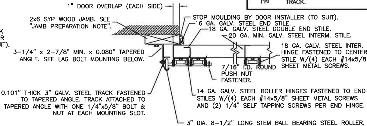
SECTION C-C
