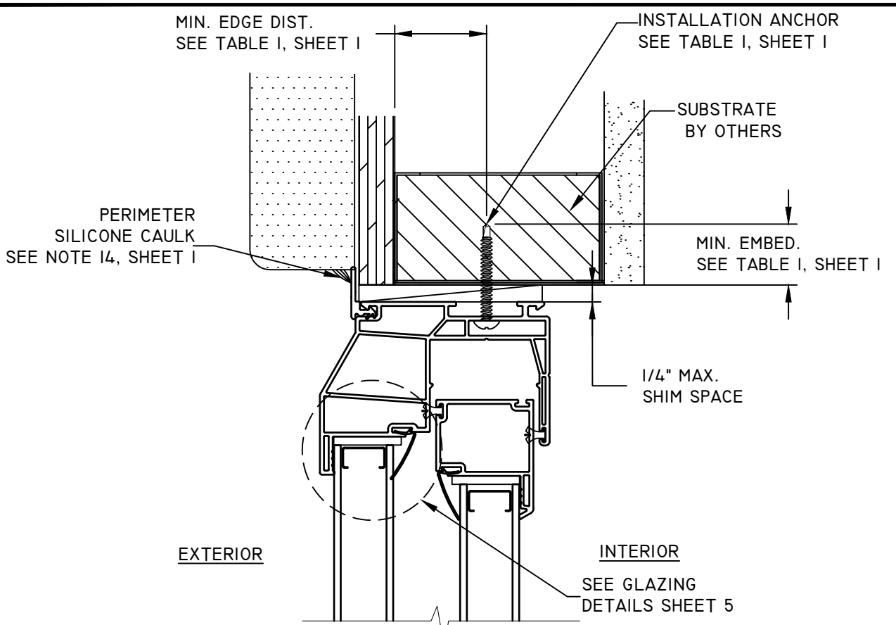
B 4 VERTICAL SECTION HEAD SHOWN - JAMB SIMILAR BEVELED FRAME - FRAME INSTALLATION
