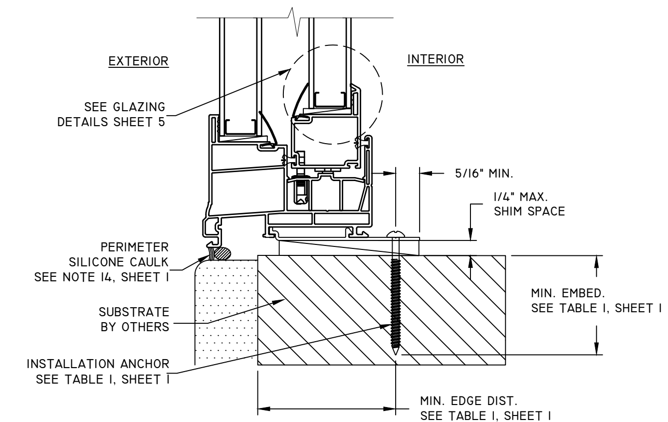
A 4 VERTICAL SECTION SILL SHOWN - HEAD/JAMB SIMILAR BRICKMOULD FRAME - CLIP INSTALLATION
