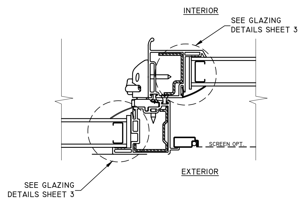
D 4 HORIZONTAL SECTION MEETING STILE TYPICAL
