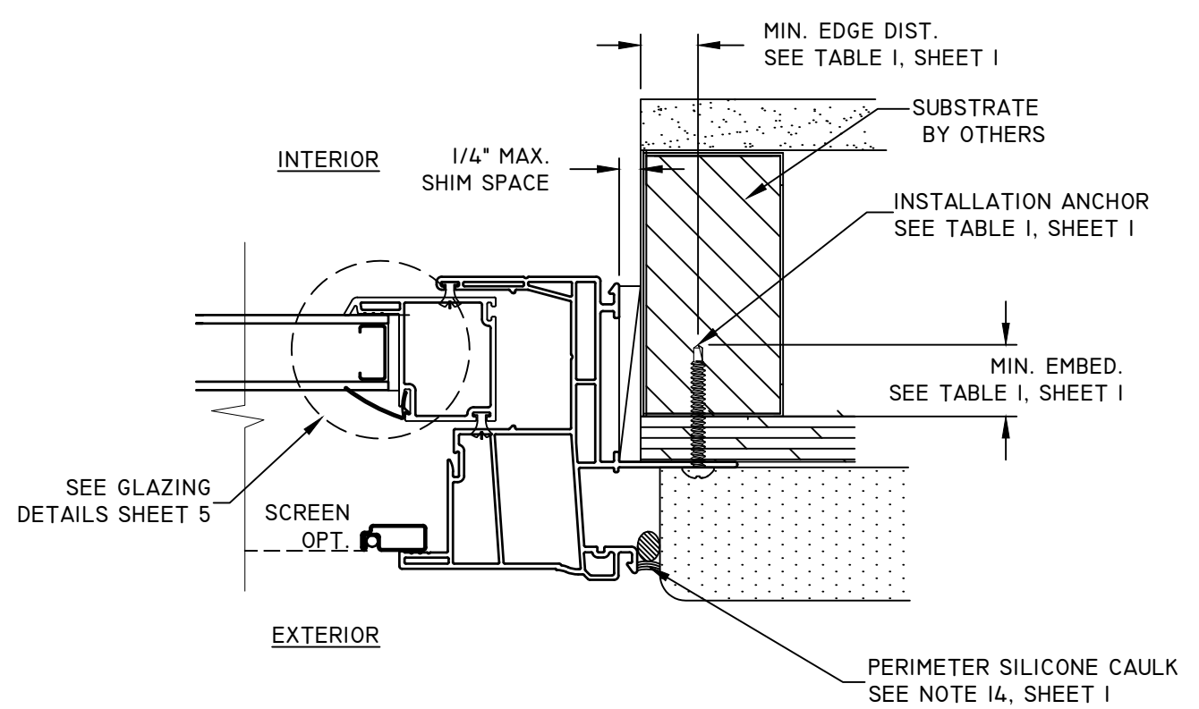
C 4 HORIZONTAL SECTION JAMB SHOWN - HEAD/SILL SIMILAR BRICKMOULD FRAME - FIN INSTALLATION
