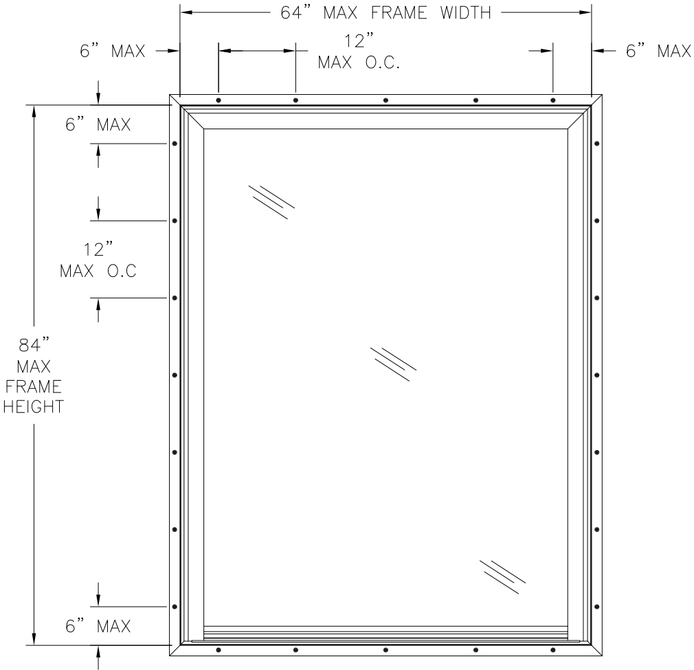
SERIES 142.000 PW EXTERIOR VIEW FIN INSTALLATION
