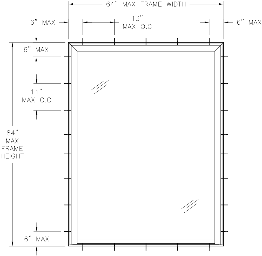
SERIES 142.000 PW EXTERIOR VIEW FRAME INSTALLATION
