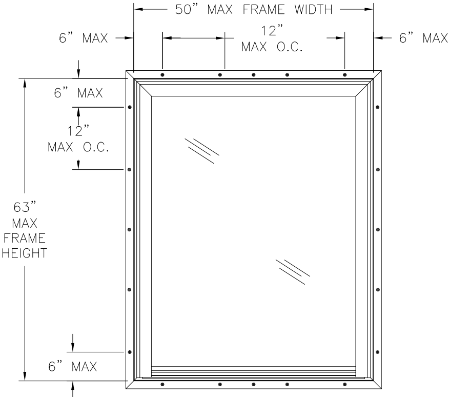
SERIES 143.000 PW EXTERIOR VIEW FIN INSTALLATION
