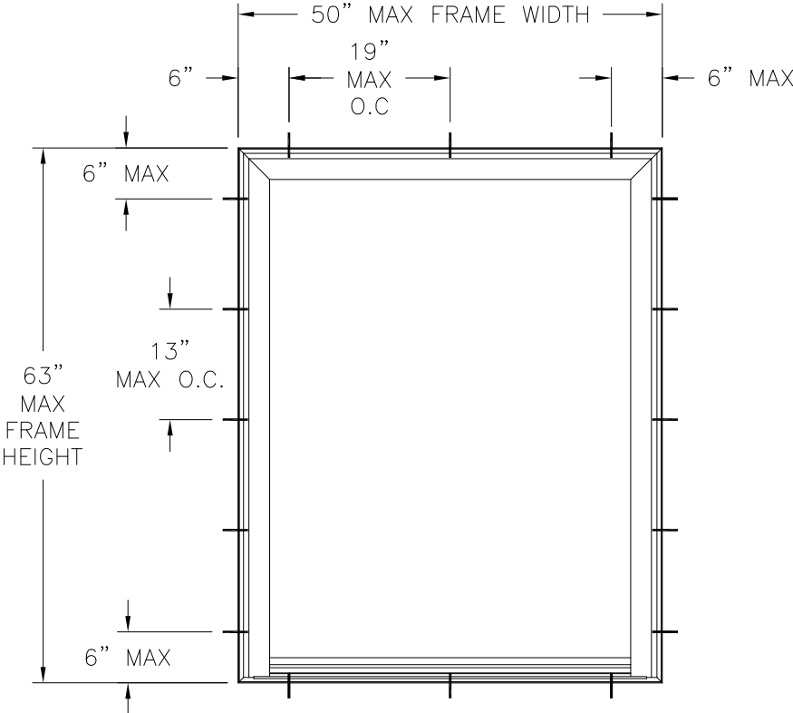
SERIES 143.000 PW EXTERIOR VIEW FRAME INSTALLATION
