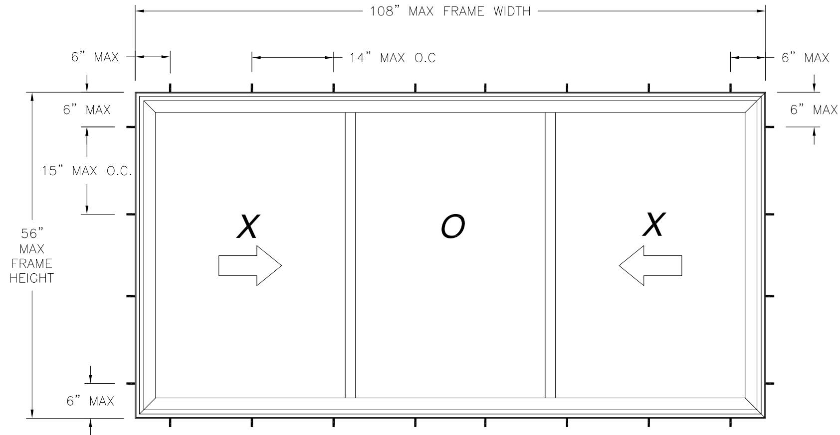
777 Protech Slider XOX (1/3 – 1/3 – 1/3) EXTERIOR VIEW
