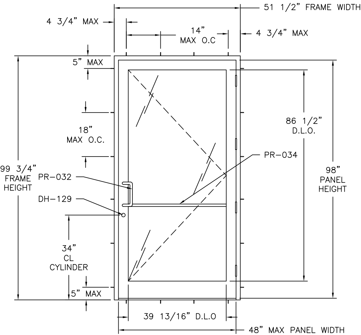
SERIES 850 ALUMINUM SINGLE DOOR EXTERIOR VIEW FRAME FLUSH INSTALLATION
