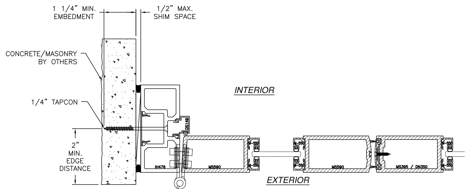
JAMB INSTALLATION DETAIL CONCRETE/MASONRY WITHOUT 1X BUCK INSTALLATION FOR CONCRETE/MASONRY WITH 1X BUCK REFER TO HEAD AND SILL INSTALLATION DETAILS
