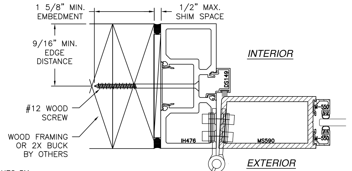
JAMB INSTALLATION DETAIL WOOD FRAMING OR 2X BUCK INSTALLATION SIGNED: 09/04/2026
