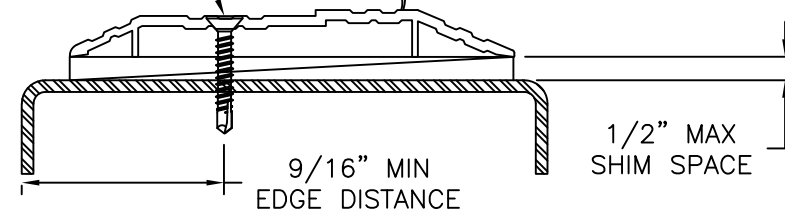
VERTICAL CROSS SECTION METAL STRUCTURE INSTALLATION
