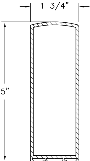
DOOR STILE ALUMINUM 6063-T5 (MS400)
