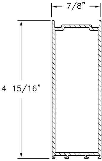
ADJUSTABLE ASTRAGAL STILE ALUMINUM 6063-T5 (MS350/DN350)
