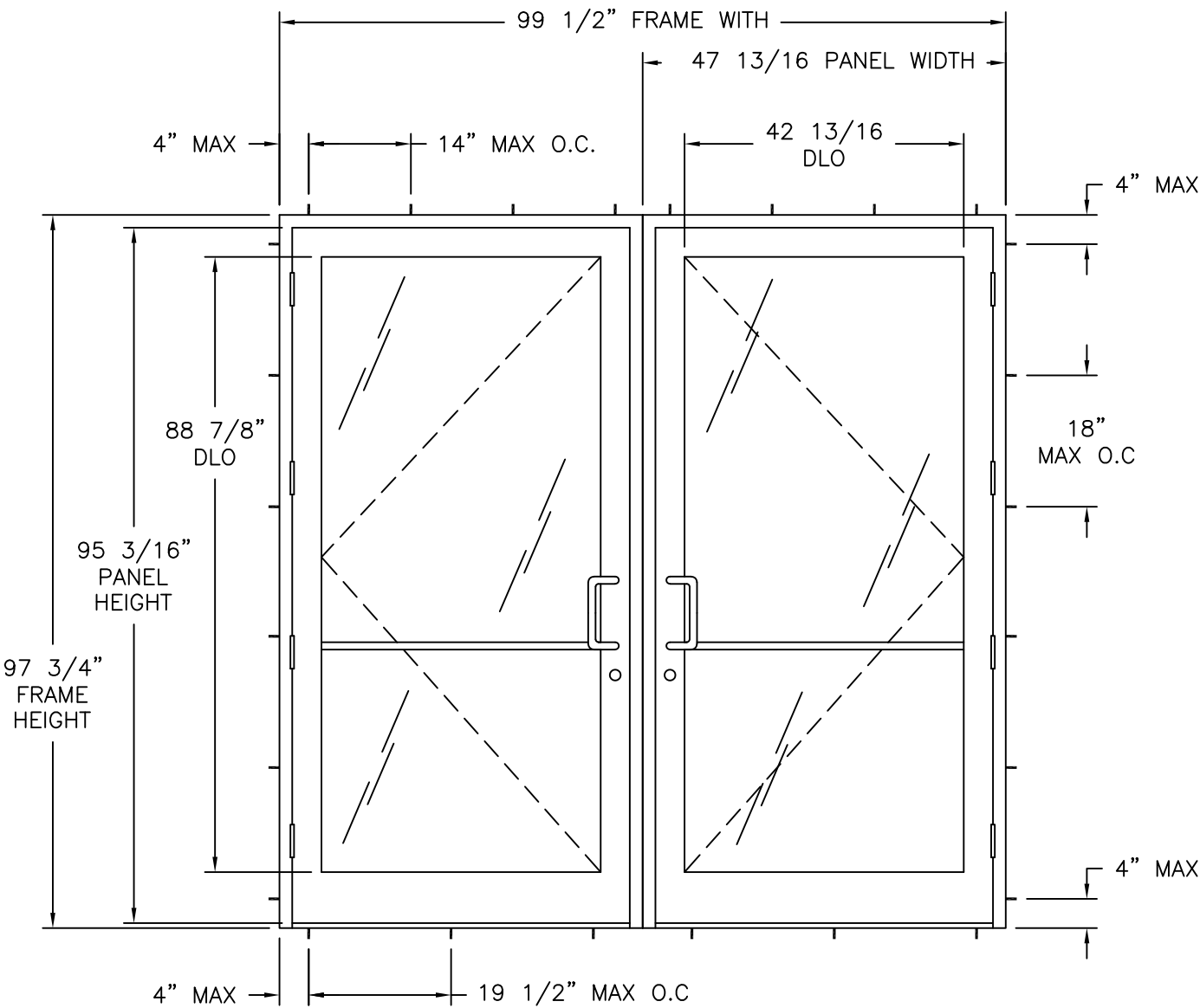
SERIES 550 ALUMINUM DOUBLE DOOR EXTERIOR VIEW
