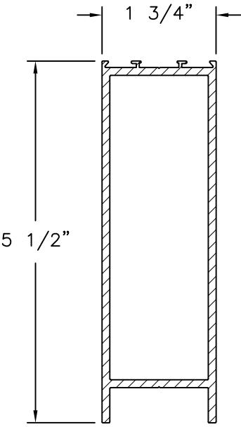
TOP RAIL ALUMINUM 6063-T5 (D101)
