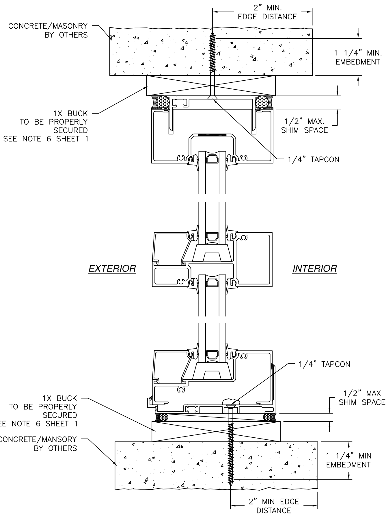
VERTICAL CROSS SECTION CONCRETE/MASONRY INSTALLATION WITH 1X BUCK INSTALLATION FOR CONCRETE/MASONRY WITHOUT 1X BUCK REFER TO JAMB INSTALLATION DETAILS
