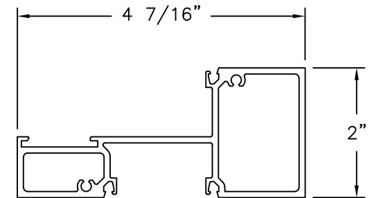
HORIZONTAL MULLION ALUMINUM 6063-T5 (IH463)
