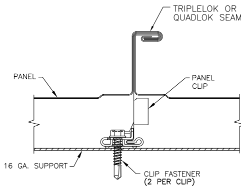
CLIP SECTION VIEW
