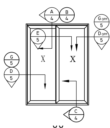
XX (NON-POCKETING DOORS) 2 TRACK
