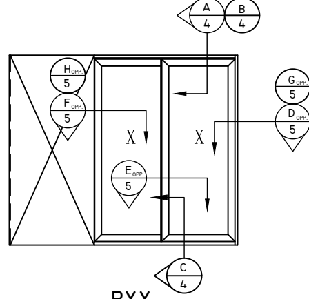
PXX (POCKETING DOORS) 2 TRACK
