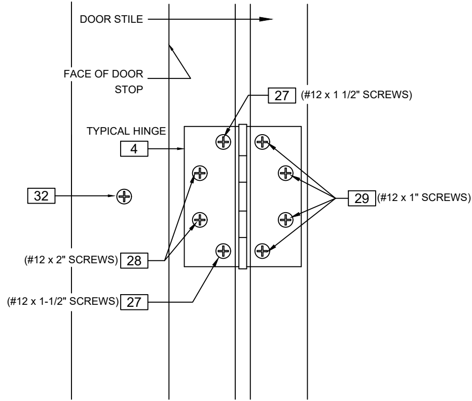
DETAIL "A". (TYPICAL AT ALL HINGES)
