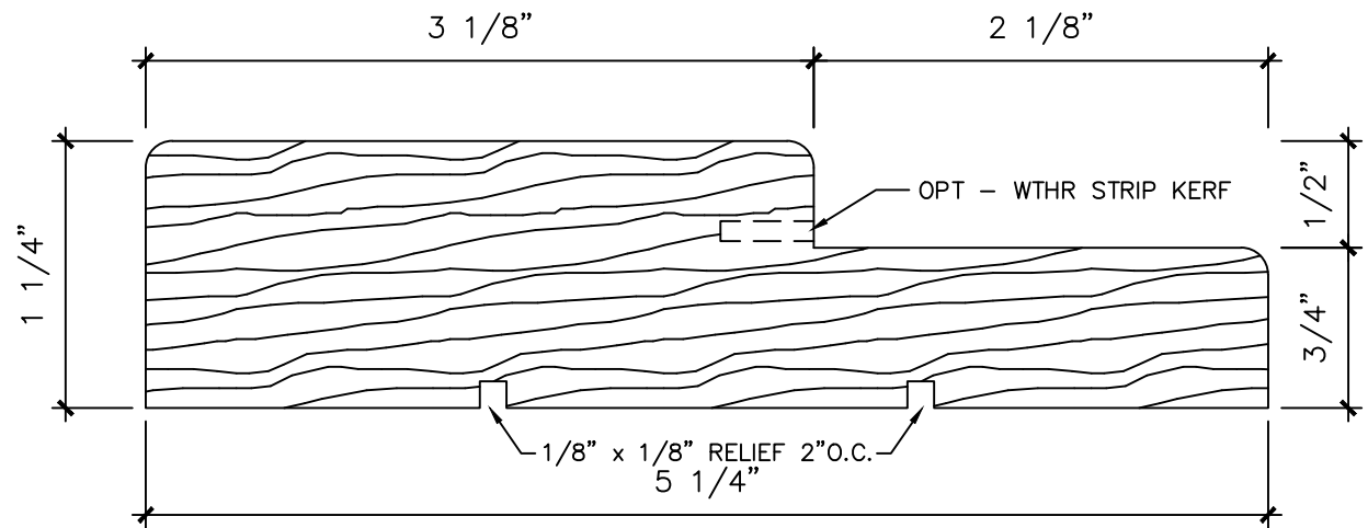
JAMB 1 SCALE: NOT TO SCALE
