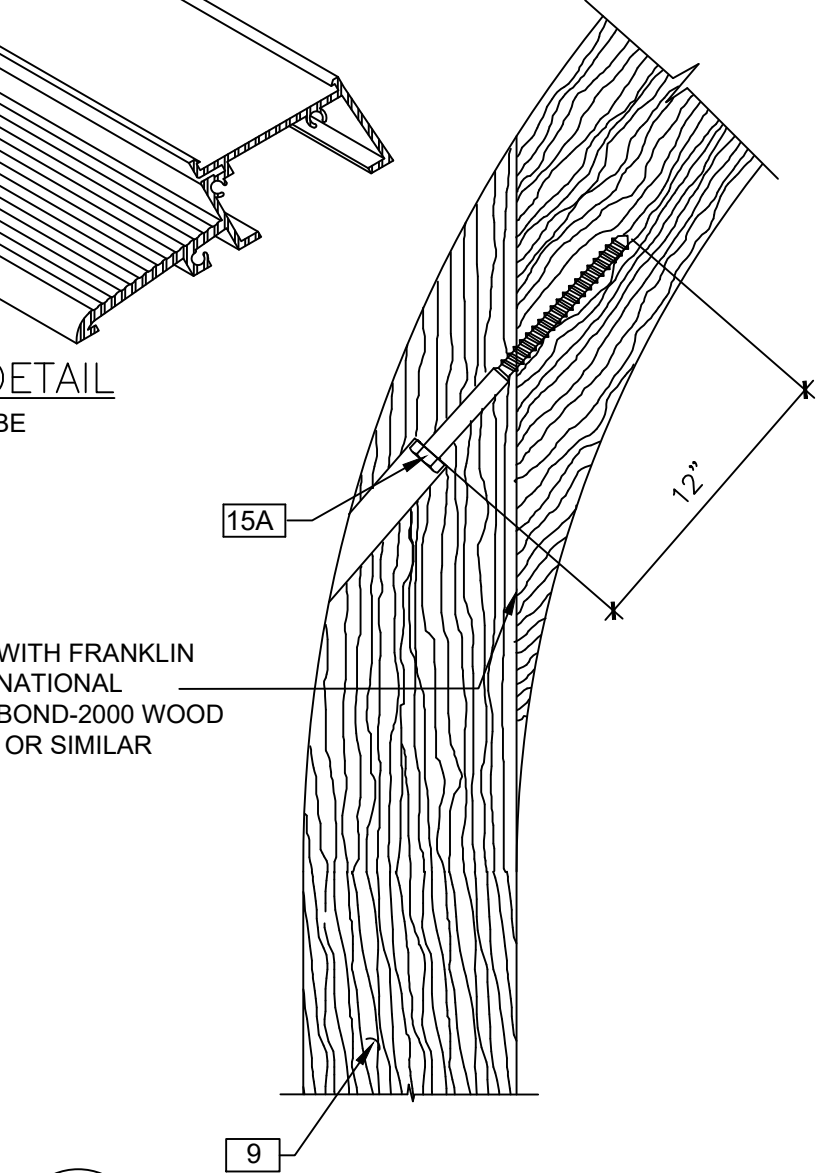
3 6 ARCHED DOOR PANEL CORNER DETAIL SCALE: 1/4" = 1"
