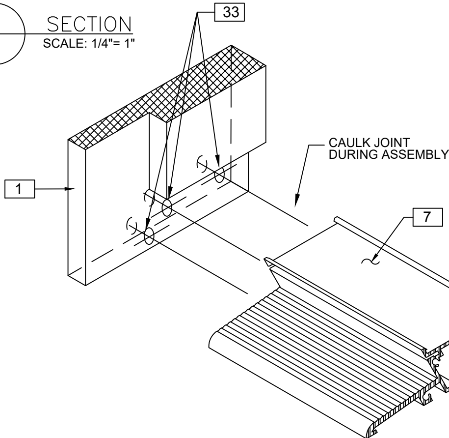
2 6 TYP. THRESHOLD CORNER DETAIL (ALL MEETING JAMB MEMBERS TO BE SCREWED AT ALL CORNERS) SCALE: NTS
