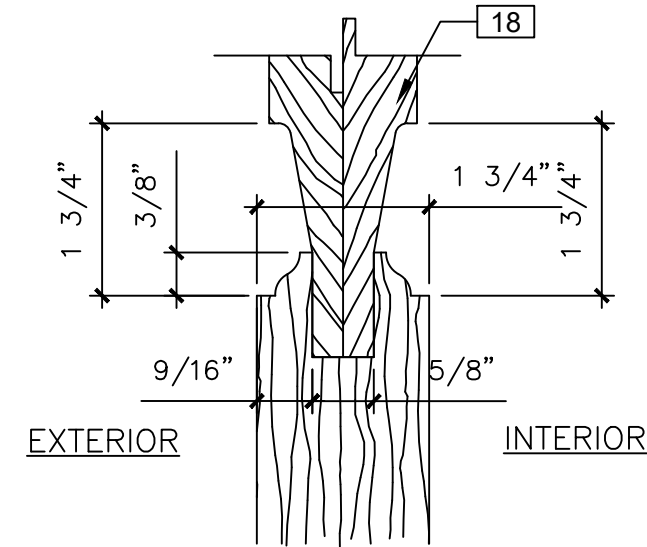
WOOD PANEL DETAIL SCALE: NTS
