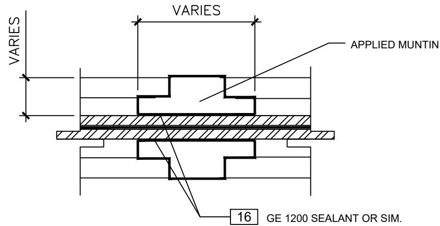
DECORATIVE SURFACE APPLIED MUNTINS SCALE: NTS
