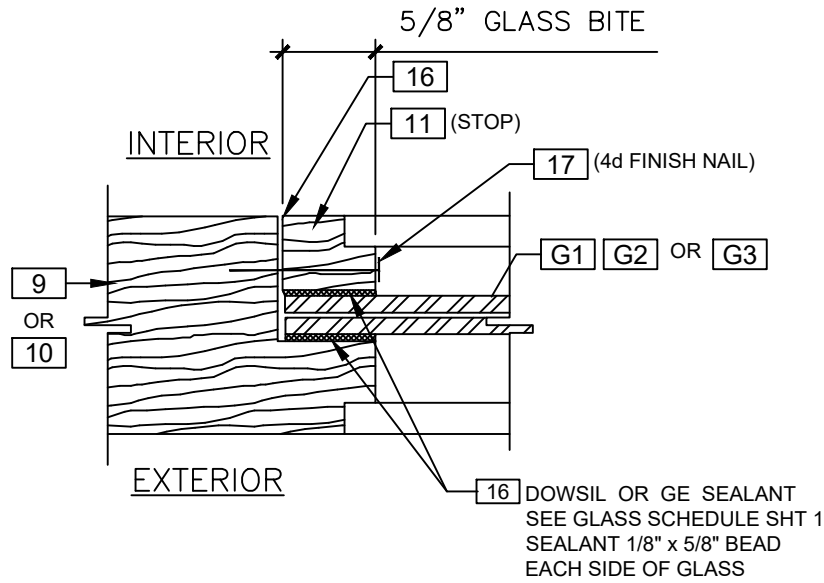
GLASS DETAIL FOR IMPACT DOORS ( 7/16" LAMINATED GLASS )
