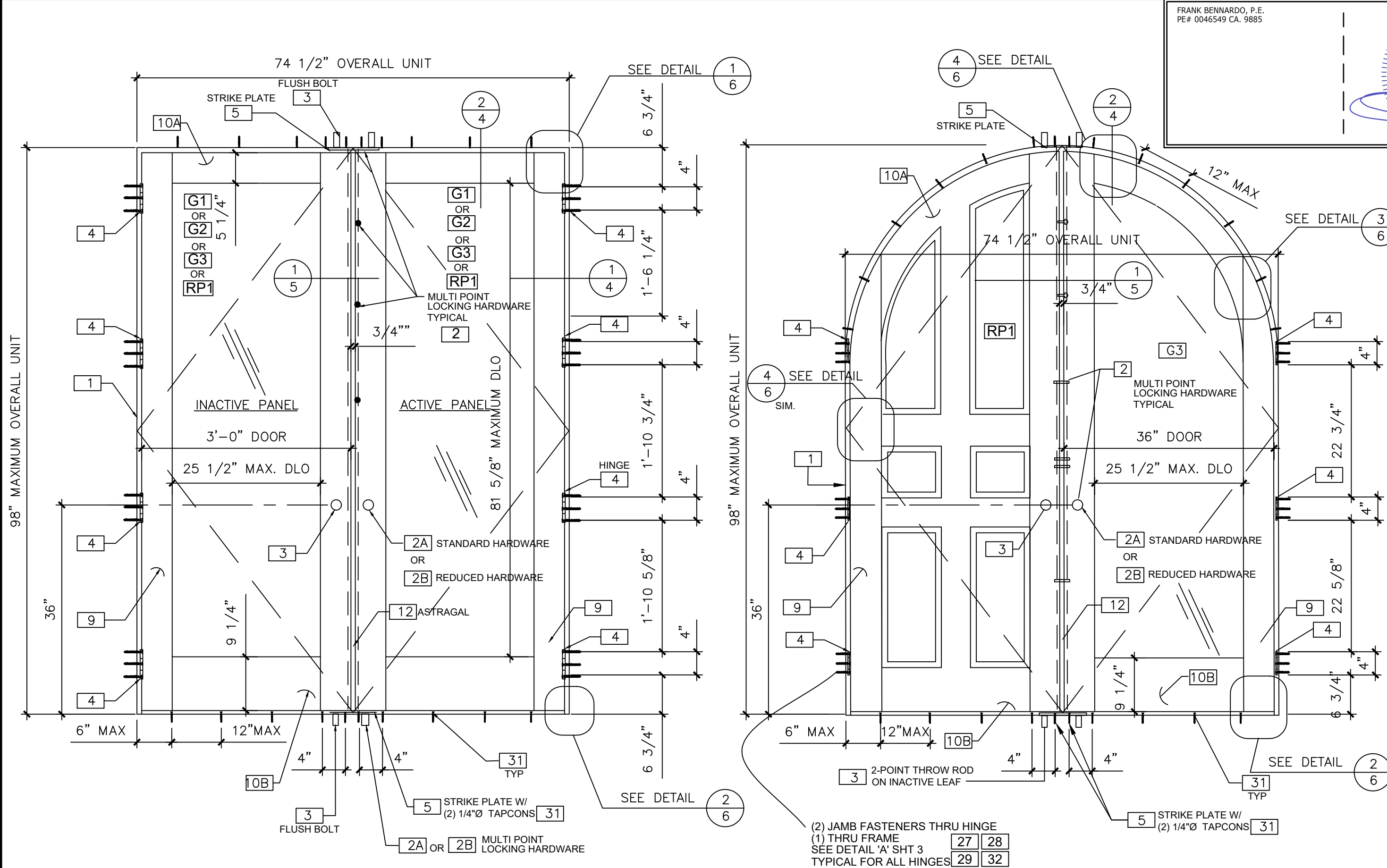
ELEVATION OF OUTSWING WOOD DOORS DOOR ASSEMBLY DETAILS (UNIT SHOWN FROM EXTERIOR) SCALE: 3/4" = 1'-0"
