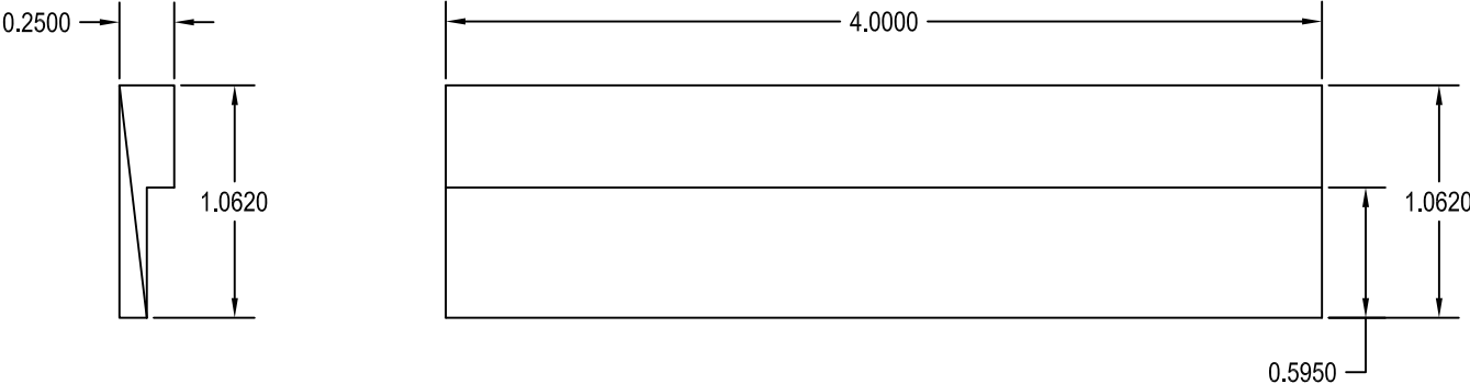
15 OFFSET SETTING BLOCK SCALE 1:1
