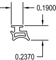
12 SILICONE GLAZING GASKET SCALE 1:1
