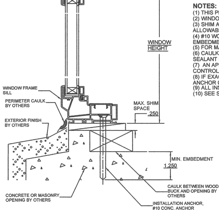
SECTION B-B
