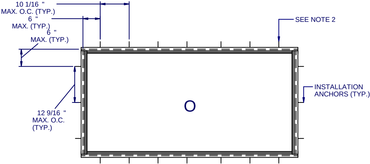
ANCHOR LAYOUT - (FLANGE) FOR UNITS RATED ±80 PSF
