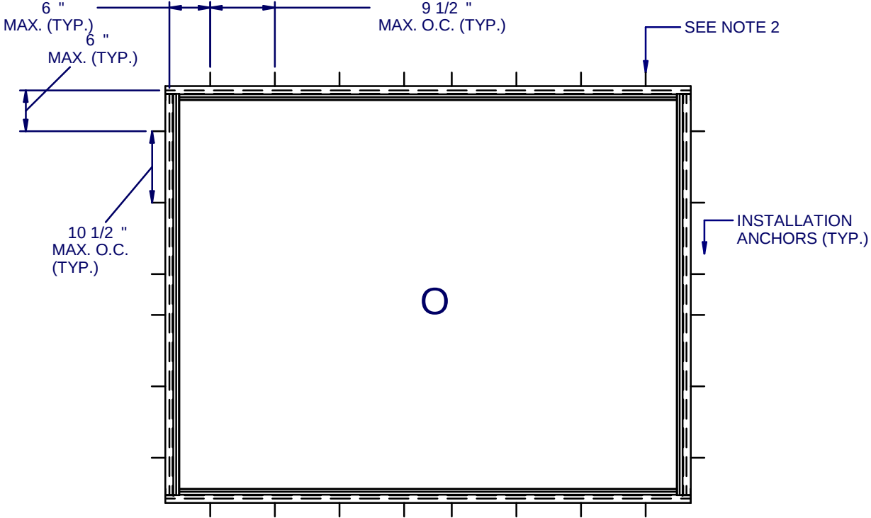
ANCHOR LAYOUT - (FLANGE) FOR UNITS RATED ±65 PSF
