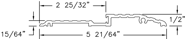
⑦ AIR SILL EXTRUDED ALUMINUM 6063-T5 .109" THICK
