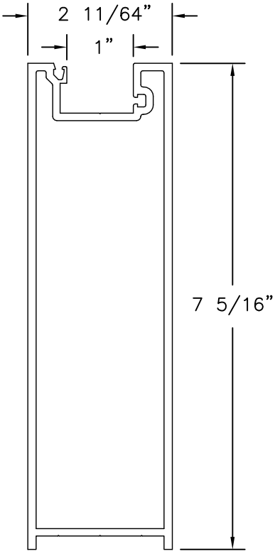
18 BOTTOM RAIL - 9/16" GLASS EXTRUDED ALUMINUM 6063-T5 .125" THICK
