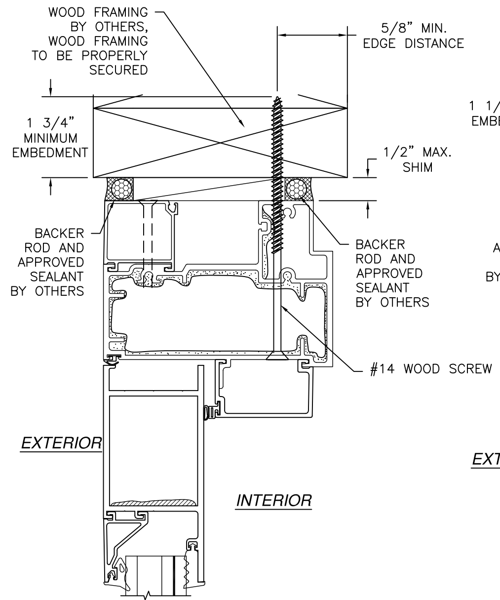
(E) OPTIONAL DOOR HEADER 2X INSTALLATION
