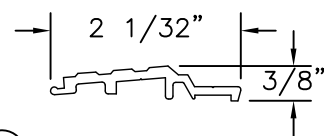
33 SILL INSERT EXTRUDED ALUMINUM 6063-T5 .090" THICK
