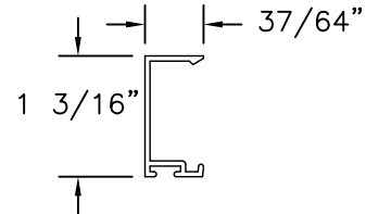
37 DOOR STOP - 9/16" GLASS EXTRUDED ALUMINUM 6063-T5 .050" THICK
