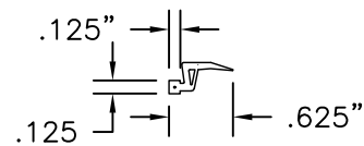
45 DOOR WEATHER STRIP VINYL
