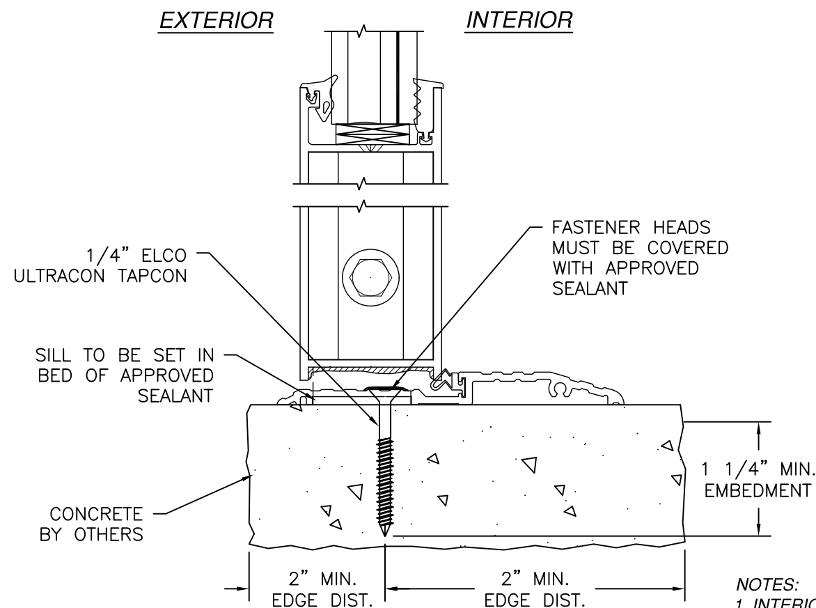
(B) AIR SILL CONCRETE INSTALLATION
