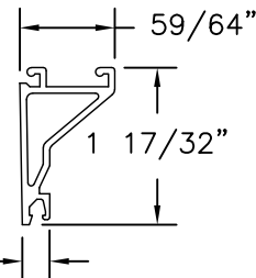
17 DOOR GLASS STOP - 1 5/16" GLASS EXTRUDED ALUMINUM 6063-T5 .062" THICK
