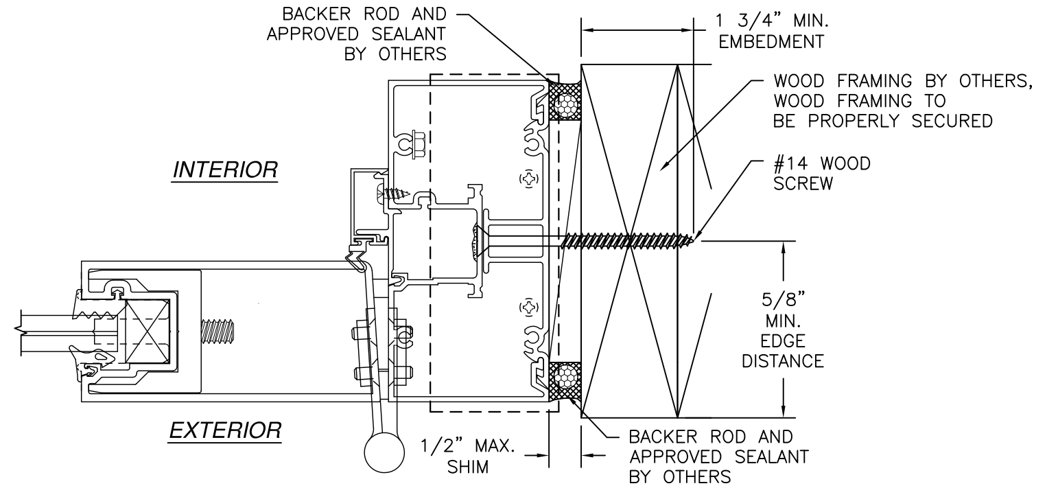
(G) JAMB WOOD FRAMING INSTALLATION HINGE JAMB SHOWN, LOCK JAMB AND TRANSOM JAMB SIMILAR
