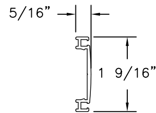
60 LOCK STILE CAP EXTRUDED ALUMINUM 6063-T5 .055" THICK
