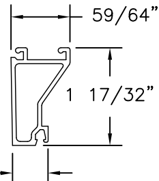
16 DOOR GLASS STOP - 9/16" GLASS EXTRUDED ALUMINUM 6063-T5 .062" THICK
