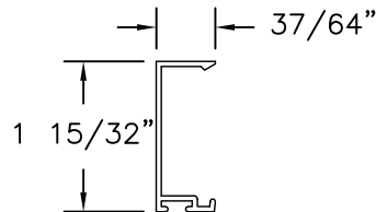
38 DOOR STOP - 1 5/16" GLASS EXTRUDED ALUMINUM 6063-T5 .050" THICK
