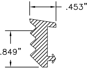
(22) INTERIOR GASKET EDPM SPONGE
