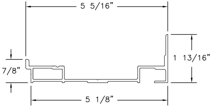
(5) SUB SILL EXTRUDED ALUMINUM 6063-T5 .075" THICK
