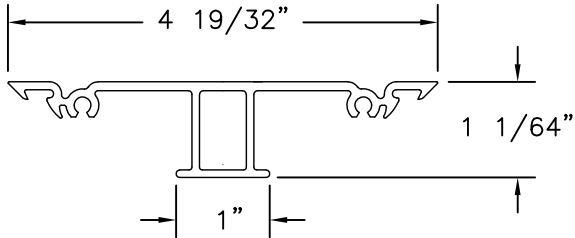
(12) FILLER JAMB/HEAD EXTRUDED ALUMINUM 6063-T5 .080" THICK
