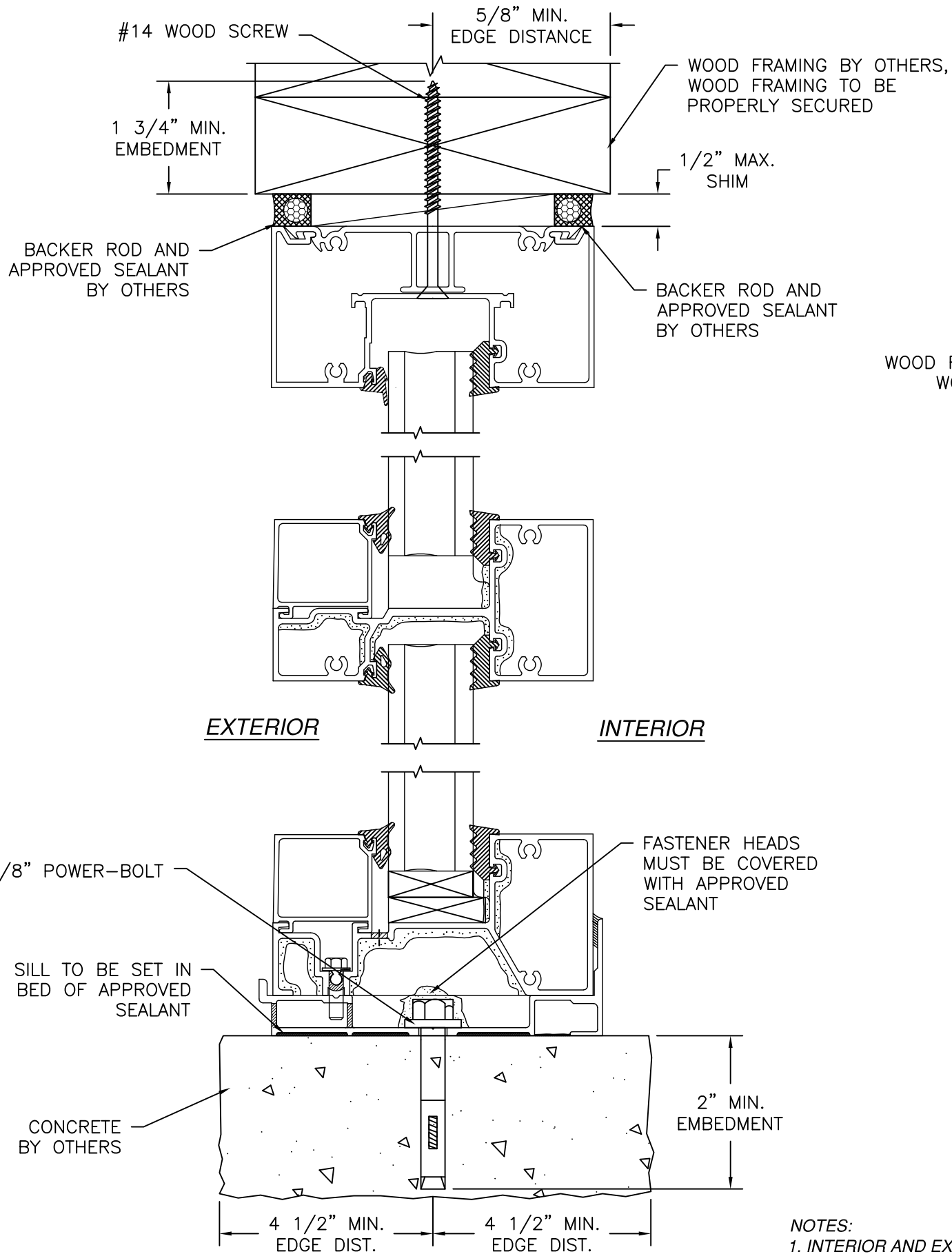
(A) HEAD & SILL INSTALLATION WOOD FRAMING AND CONCRETE
