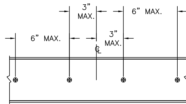
HEAD CLUSTER DETAIL CONCRETE INSTALATION
