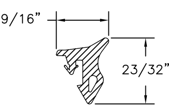
(21) EXTERIOR GASKET 70 DUROMETER EDPM
