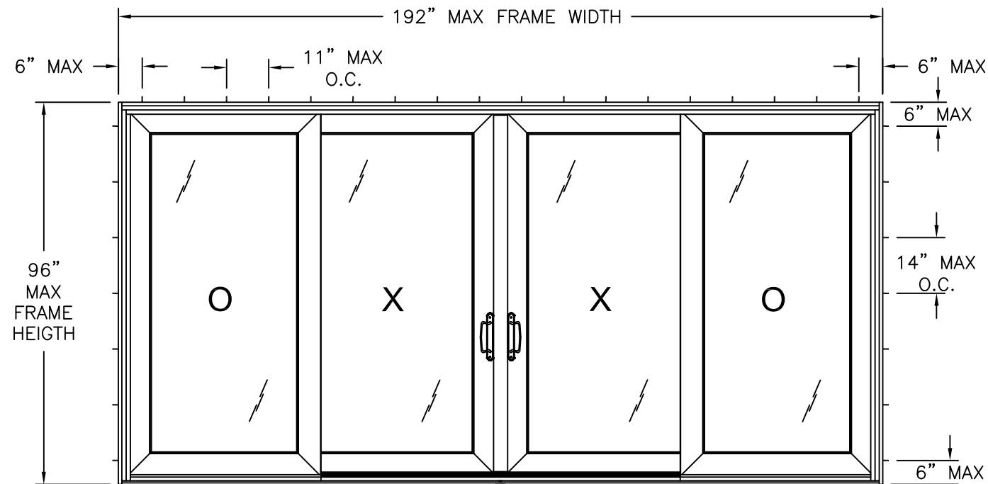
OCEANVIEW IMPACT PATIO DOOR EXTERIOR VIEW FRAME INSTALLATION
