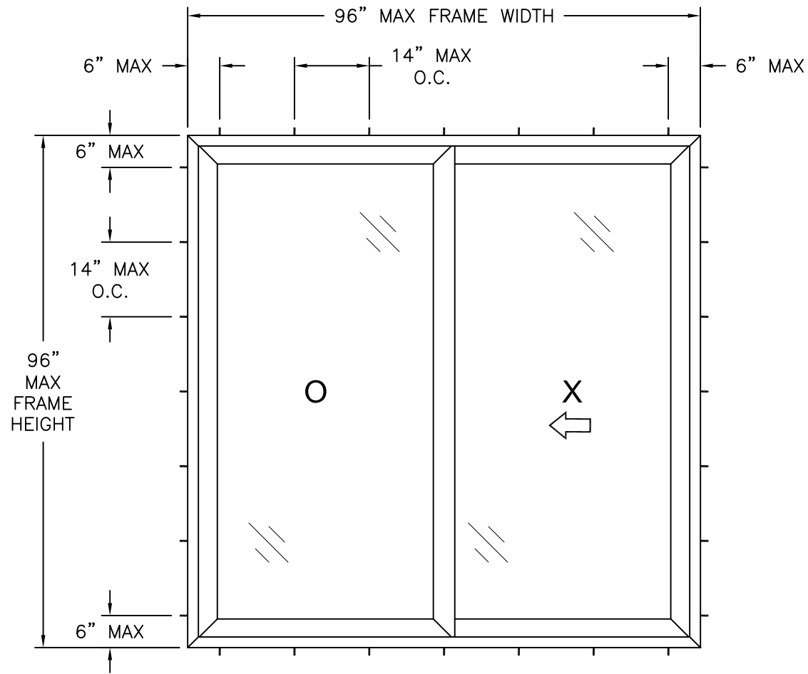
623.620PD-004 IMPACT PATIO DOOR EXTERIOR VIEW FRAME INSTALLATION
