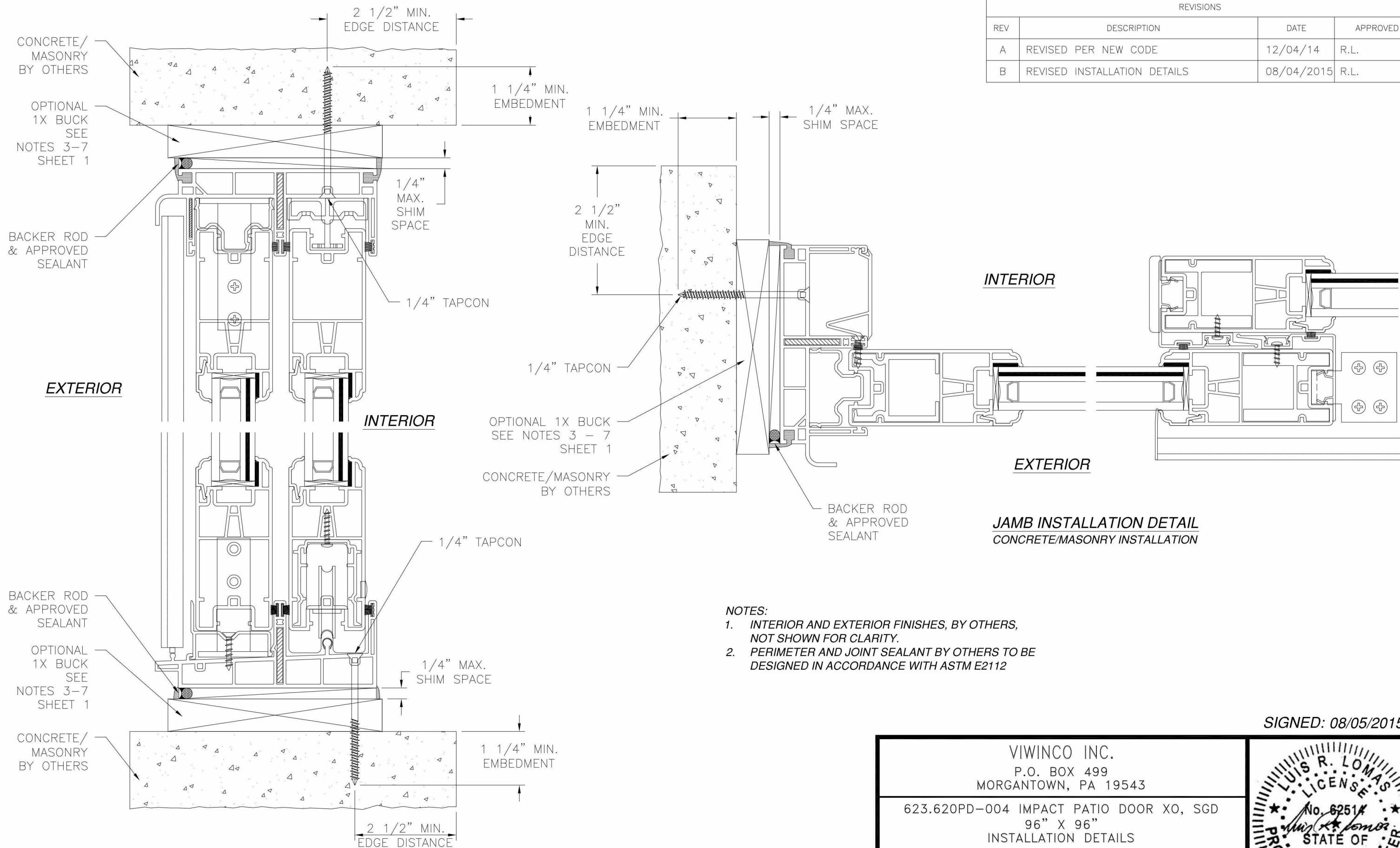
VERTICAL CROSS SECTION CONCRETE/MASONRY INSTALLATION
