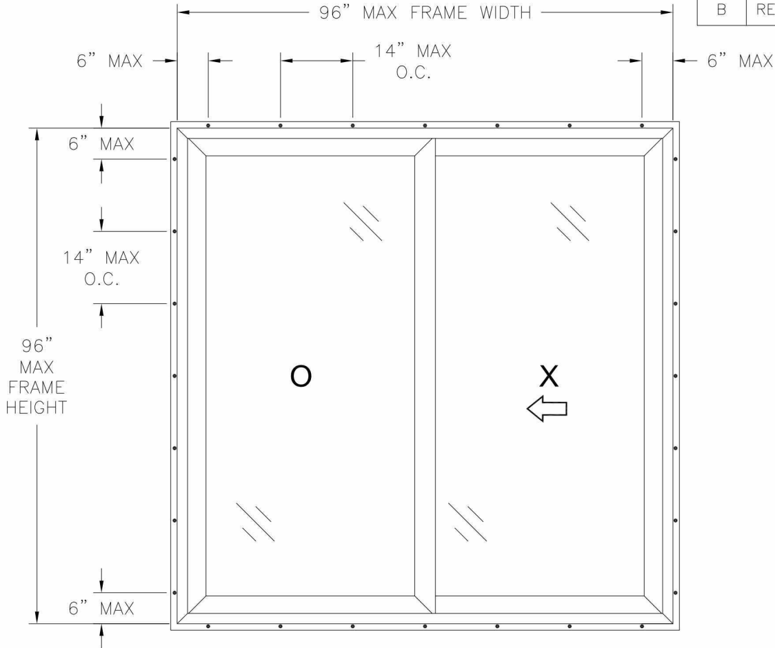
623.620PD-004 IMPACT PATIO DOOR EXTERIOR VIEW FIN INSTALLATION
