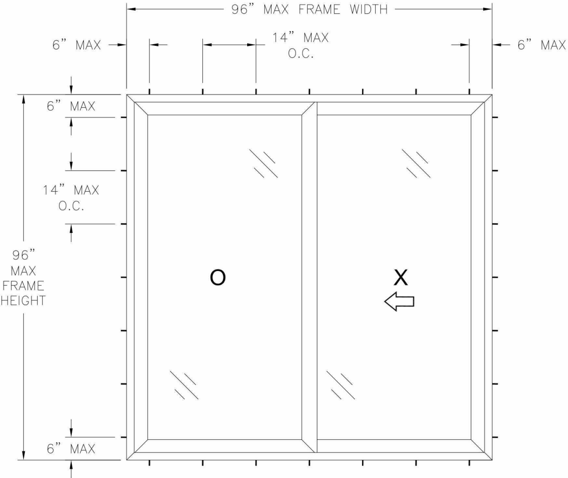
623.620PD-004 IMPACT PATIO DOOR EXTERIOR VIEW FRAME INSTALLATION
