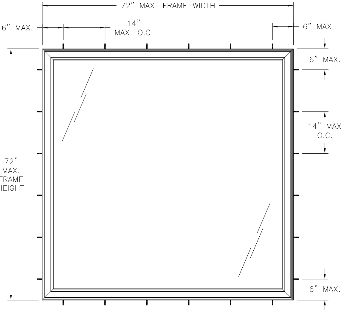
OCEANVIEW CASEMENT PICTURE EXTERIOR VIEW FRAME INSTALLATION
