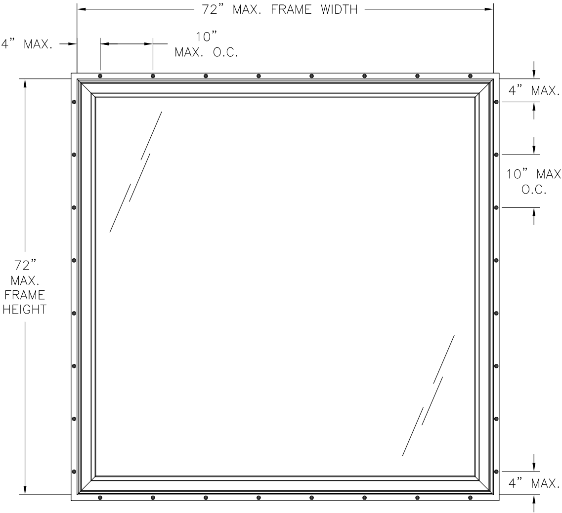
OCEANVIEW CASEMENT PICTURE EXTERIOR VIEW FIN INSTALLATION
