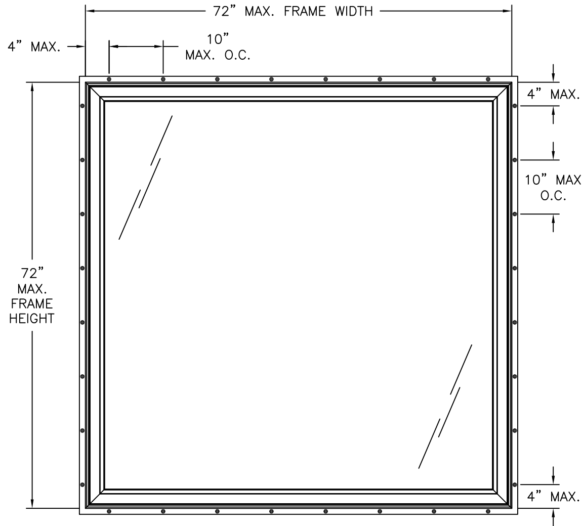
OCEANVIEW CASEMENT PICTURE EXTERIOR VIEW FIN INSTALLATION
