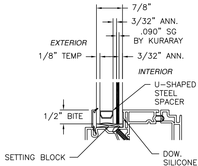
GLAZING DETAIL A
