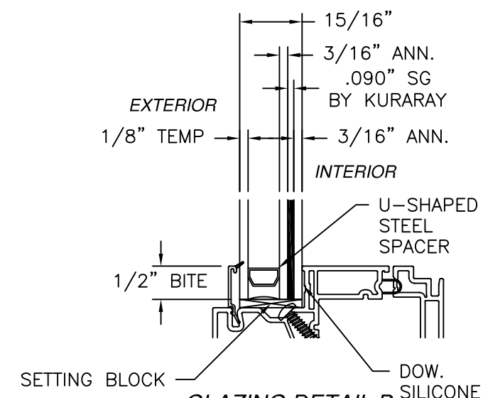
GLAZING DETAIL B
