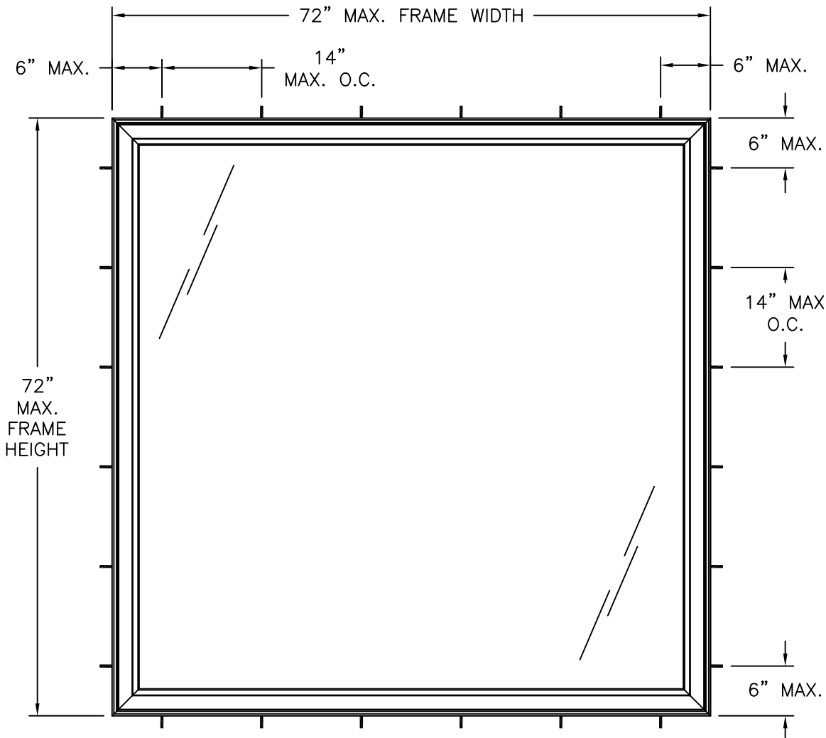
OCEANVIEW CASEMENT PICTURE EXTERIOR VIEW FRAME INSTALLATION
