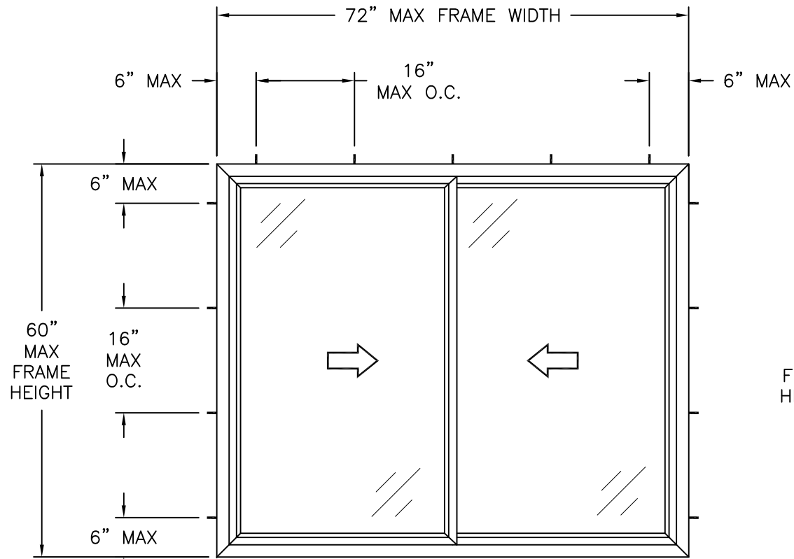
OCEANVIEW IMPACT HORIZONTAL SLIDER EXTERIOR VIEW FRAME INSTALLATION
