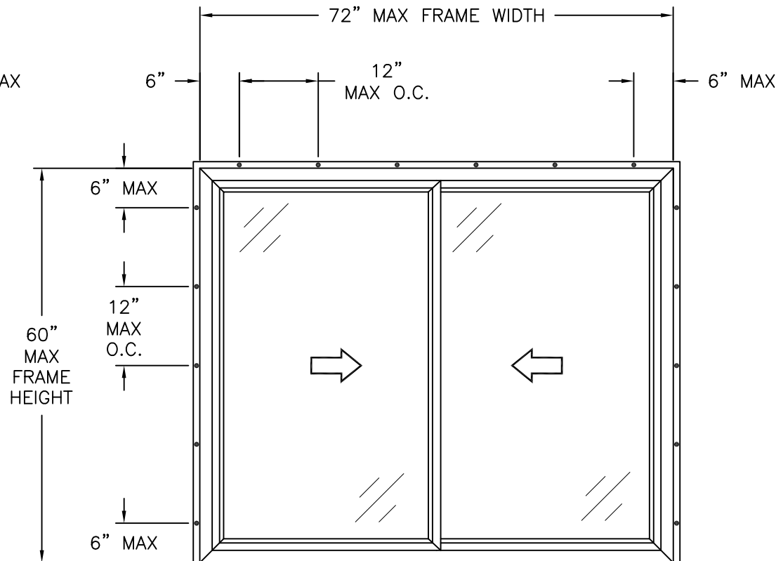
OCEANVIEW IMPACT HORIZONTAL SLIDER EXTERIOR VIEW FIN INSTALLATION
