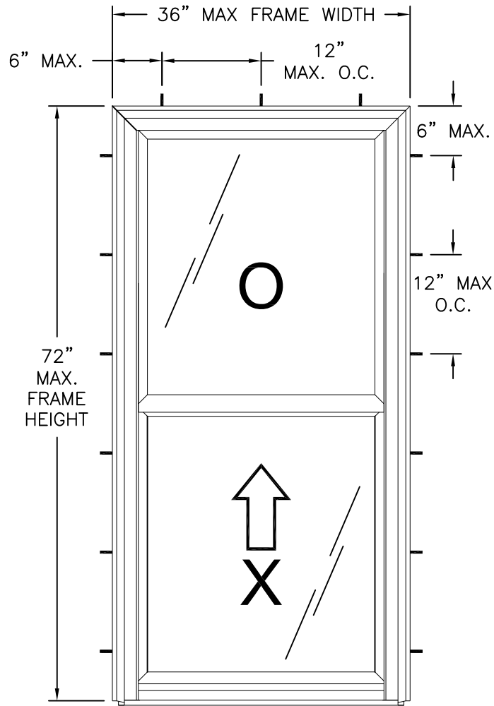
OCEANVIEW SINGLE HUNG WINDOW EXTERIOR VIEW FRAME FLUSH INSTALLATION
