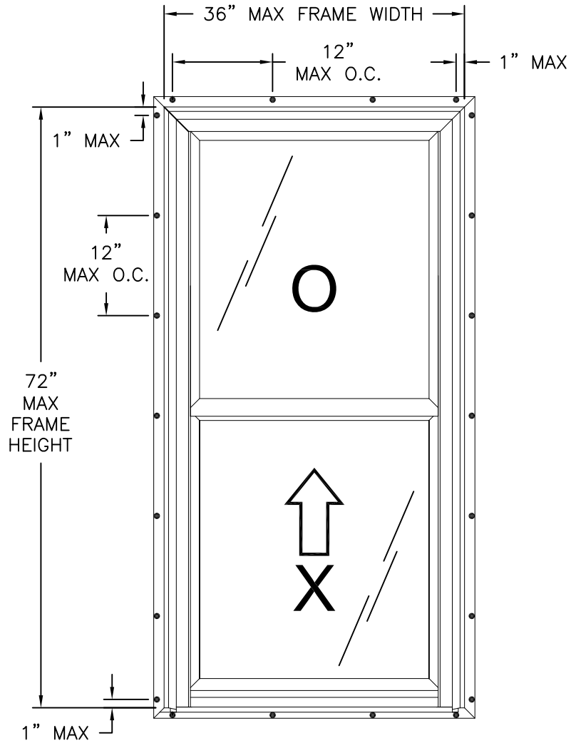
OCEANVIEW SINGLE HUNG WINDOW EXTERIOR VIEW FIN INSTALLATION
