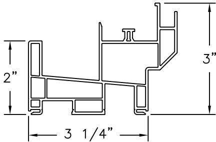
Frame Head VINYL PVC .069 THICK
