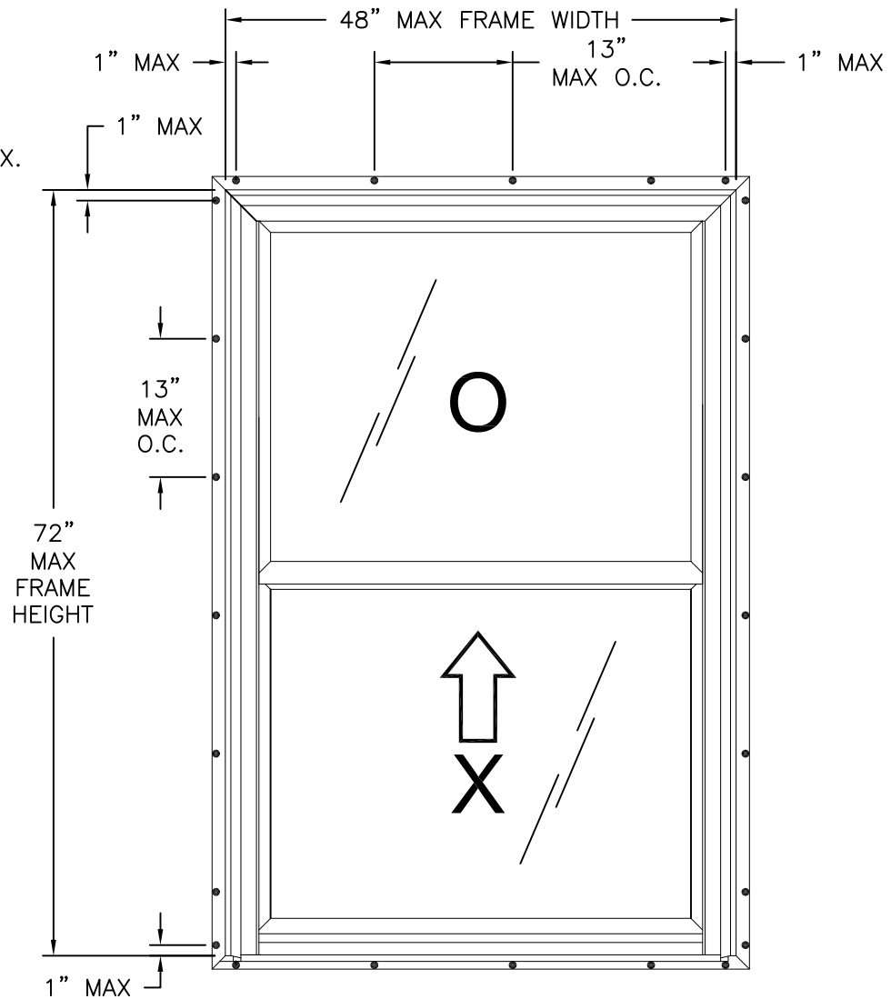
OCEANVIEW SINGLE HUNG WINDOW EXTERIOR VIEW FIN INSTALLATION
