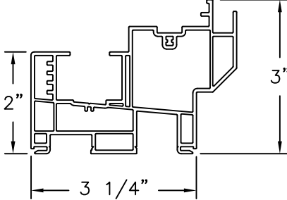
Frame Jambs VINYL PVC .069 THICK
