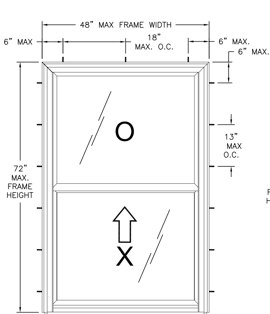
OCEANVIEW SINGLE HUNG WINDOW EXTERIOR VIEW FRAME FLUSH INSTALLATION
