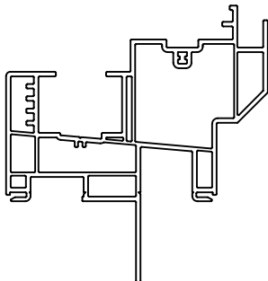
Frame Jambs (Nailing Fin) VINYL PVC .069 THICK
