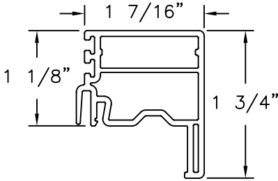
Lower Sash Meeting Rail VINYL PVC .059 THICK
