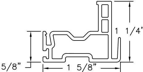
Upper Sash Meeting Rail VINYL PVC .059 THICK
