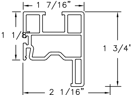
Top Sash Rail VINYL PVC .059 THICK
