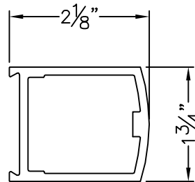
ITEM 8 - E0056 NARROW ROUND FACE STILE
