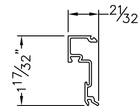
ITEM 11 - E0437 GLASS STOP
