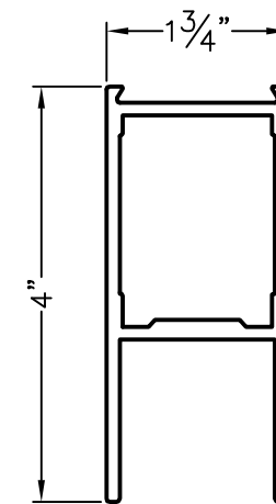
ITEM 5 - E0054 BOTTOM RAIL
