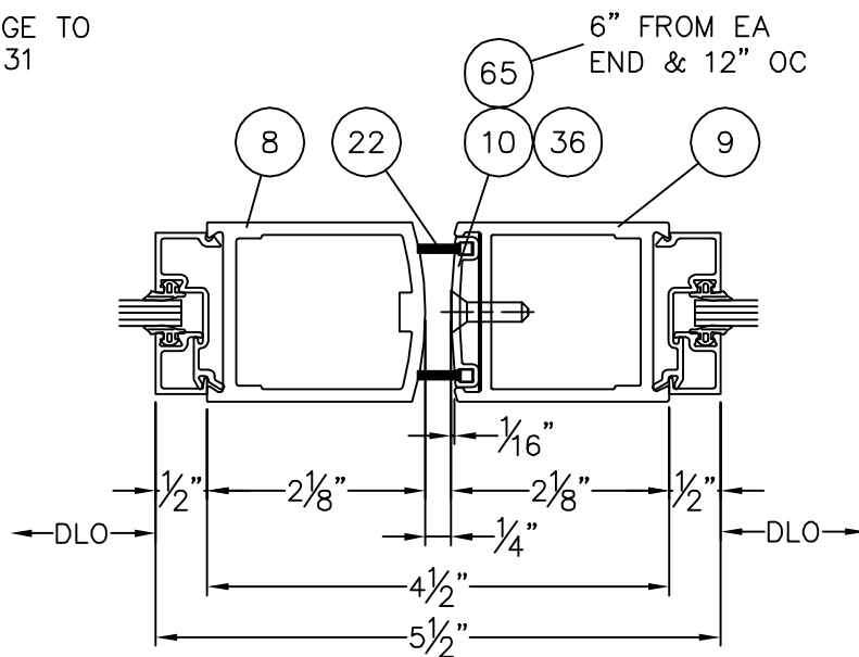
4 4 ASTAGAL NARROW STILE
