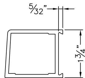
ITEM 7 - E0055 NARROW STILE BUTT HINGE
