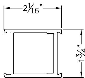
ITEM 9 - E1149 NARROW STILE LOCK W/ASTRAGAL
