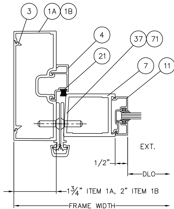
2A 4 JAMB W/CONTINUOUS HINGE NARROW STILE
