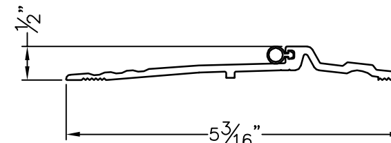
ITEM 20 - P6513-OR THRESHOLD
