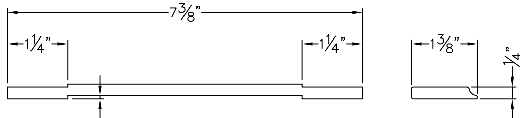
ITEM 31 - P1218 BUTT HINGE REINFORCEMENT
