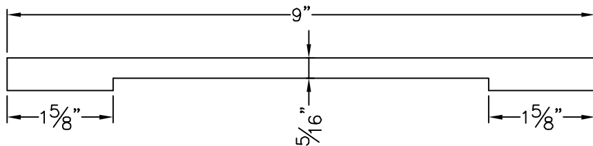
ITEM 43 - P0360 INTERMEDIATE PIVOT REINFORCEMENT
