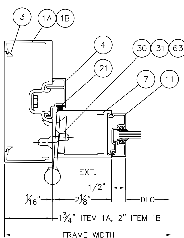
2C 4 JAMB W/BUTT HINGE NARROW STILE
