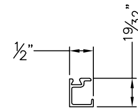
ITEM 12 - E0410 SNAP IN GLASS STOP
