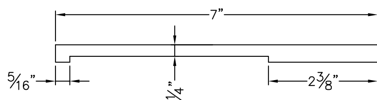
ITEM 55 TOP PIVOT REINFORCEMENT
