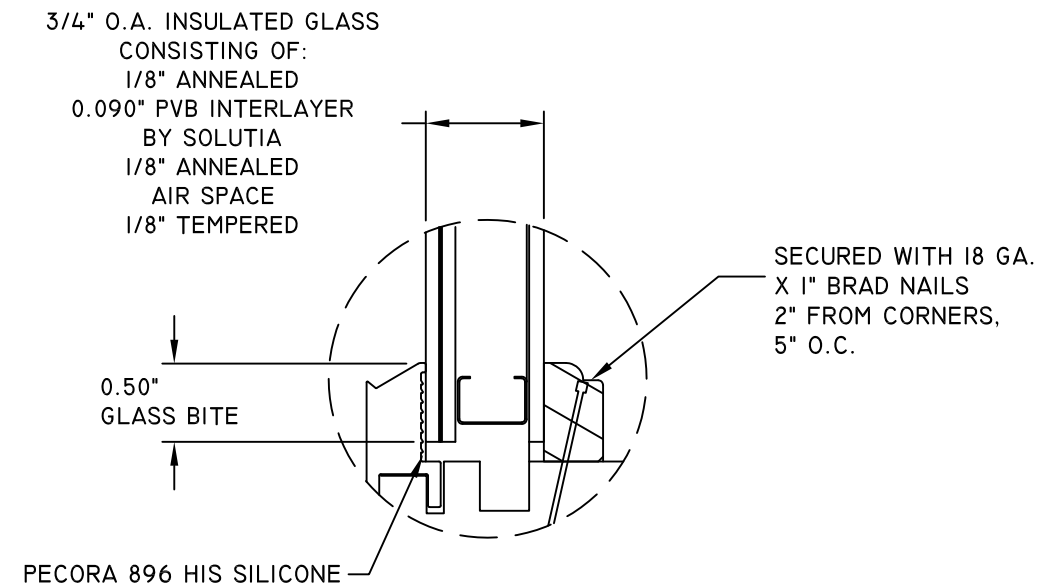
GLAZING DETAIL 1
