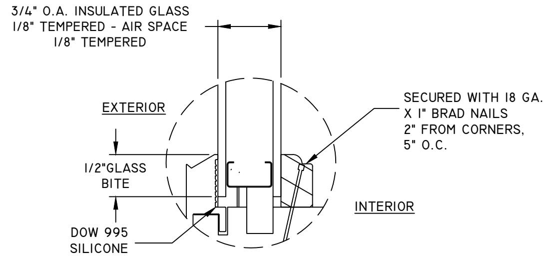
GLAZING DETAIL 1
