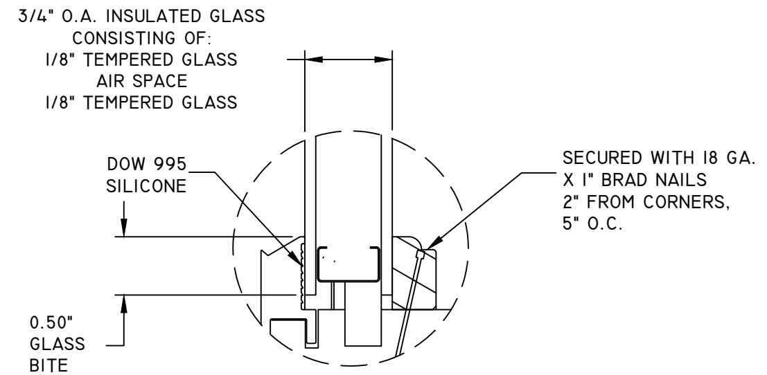
GLAZING DETAIL 1
