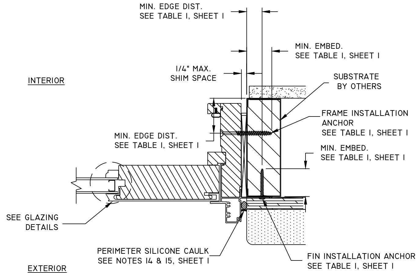
C 4 HORIZONTAL SECTION FIXED PANEL
