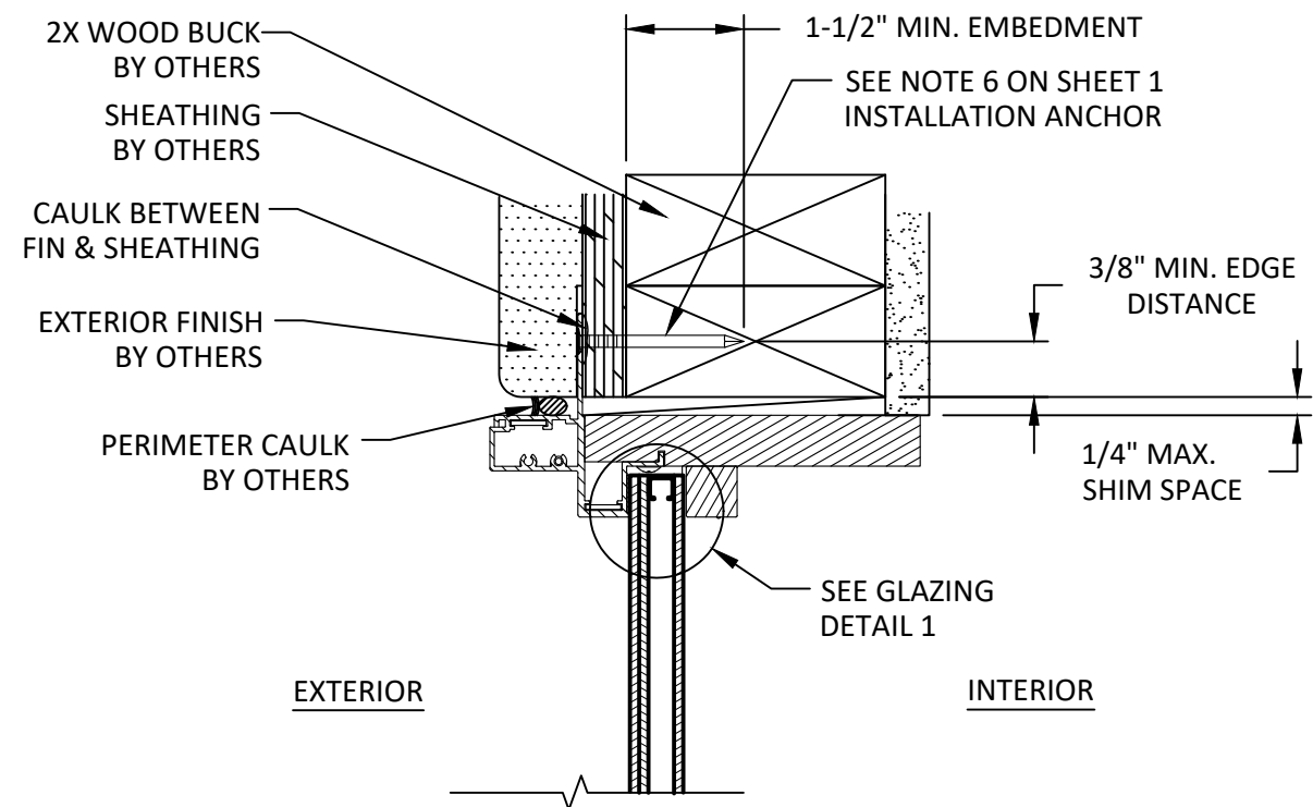
B 3 VERTICAL SECTION 2X WOOD FRAME - HEAD FIN INSTALLATION
