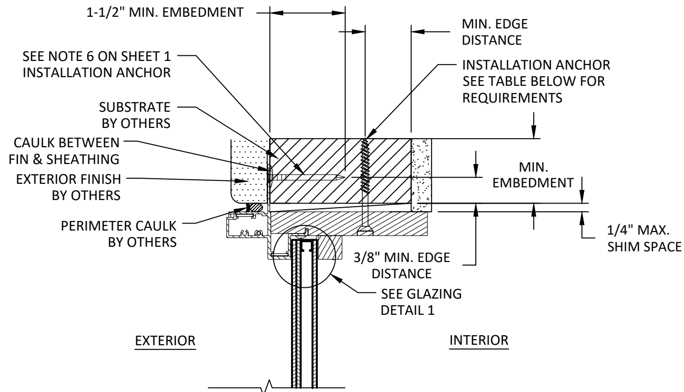
C 3 VERTICAL SECTION THROUGH FRAME INSTALLATION REQUIRED AT 4" FROM CORNERS AND MIDSPAN IN ADDITION TO NAIL FIN ANCHORS FOR SIZES OVER 49-3/8" X 76-9/16"
