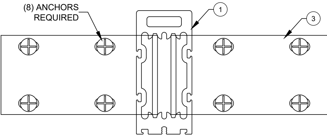
BRACKET (3418) TO MULLION DETAILS (WOOD ANCHOR INSTALLATION)
