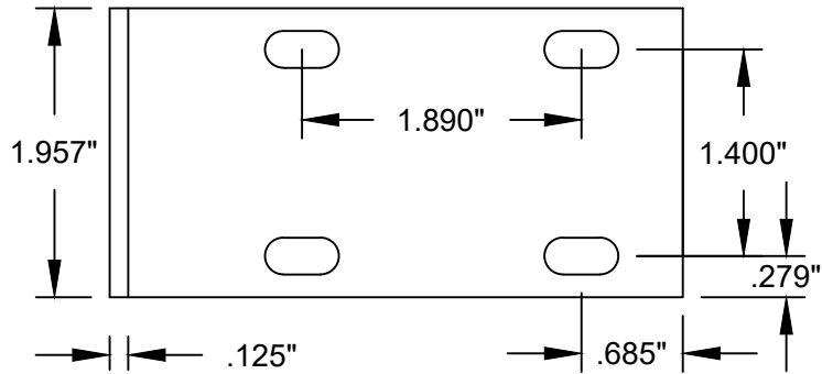
2 MULLION ANCHOR BRACKET (3419) (6063-T6 ALUMINUM)
