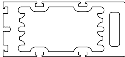
① 6225 MULLION (6063-T6 ALUMINUM)
