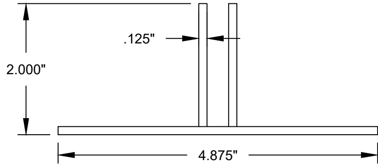
2 MULLION ANCHOR BRACKET (3419) (6063-T6 ALUMINUM)
