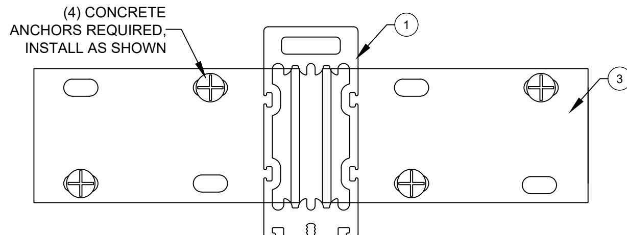
BRACKET (3418) TO MULLION DETAILS (HOLLOW BLOCK OR 3K CONCRETE ANCHOR INSTALLATION)
