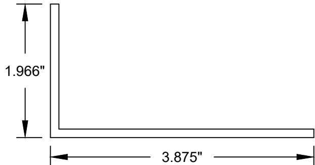
3 MULLION ANCHOR BRACKET (3418) (6063-T6 ALUMINUM)
