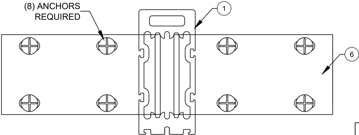
BRACKET (3418) TO MULLION DETAILS (HOLLOW BLOCK OR 3K CONCRETE ANCHOR INSTALLATION)
