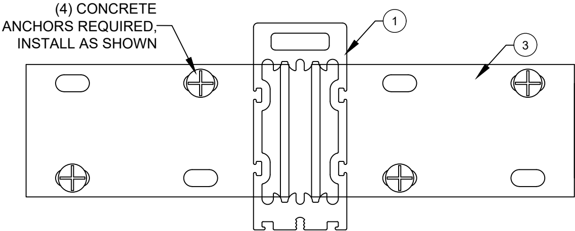
BRACKET (3418) TO MULLION DETAILS (HOLLOW BLOCK & 3K CONCRETE ANCHOR INSTALLATION)
