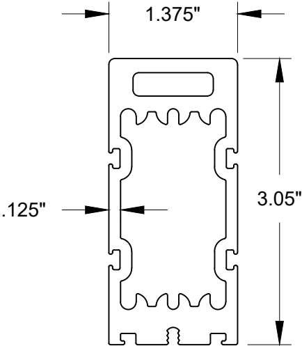
1 6225 MULLION (6063-T6 ALUMINUM)
