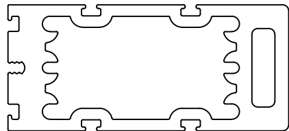
1 6225 MULLION (6063-T6 ALUMINUM)
