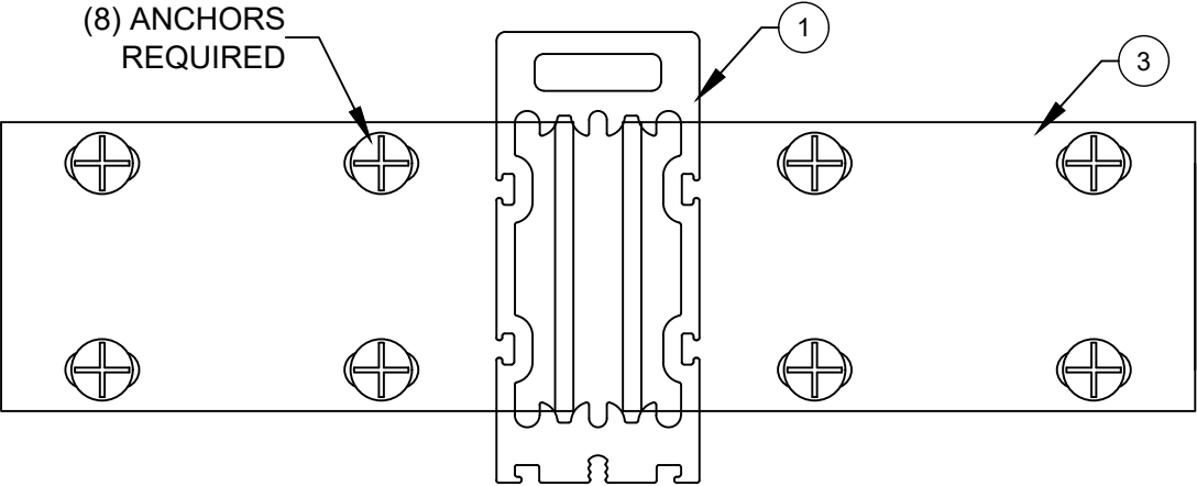
BRACKET (3418) TO MULLION DETAILS (HOLLOW BLOCK OR 3K CONCRETE ANCHOR INSTALLATION)
