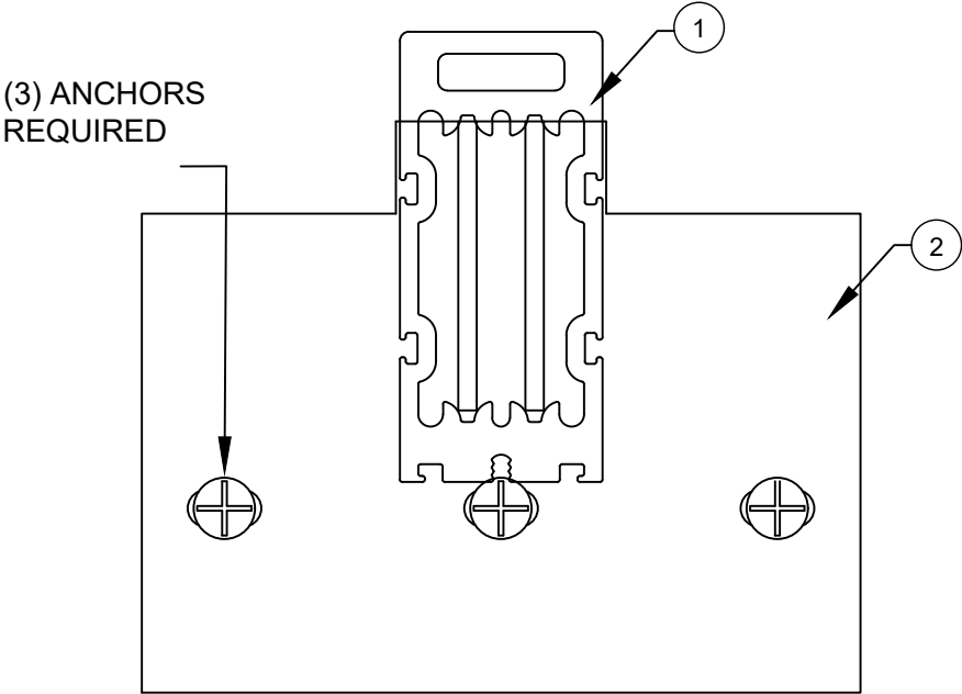
BRACKET (3419) TO MULLION DETAILS (HOLLOW BLOCK OR 3K CONCRETE ANCHOR INSTALLATION)
