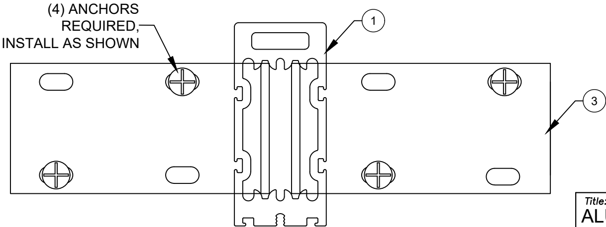
BRACKET (3418) TO MULLION DETAILS (WOOD ANCHOR INSTALLATION)
