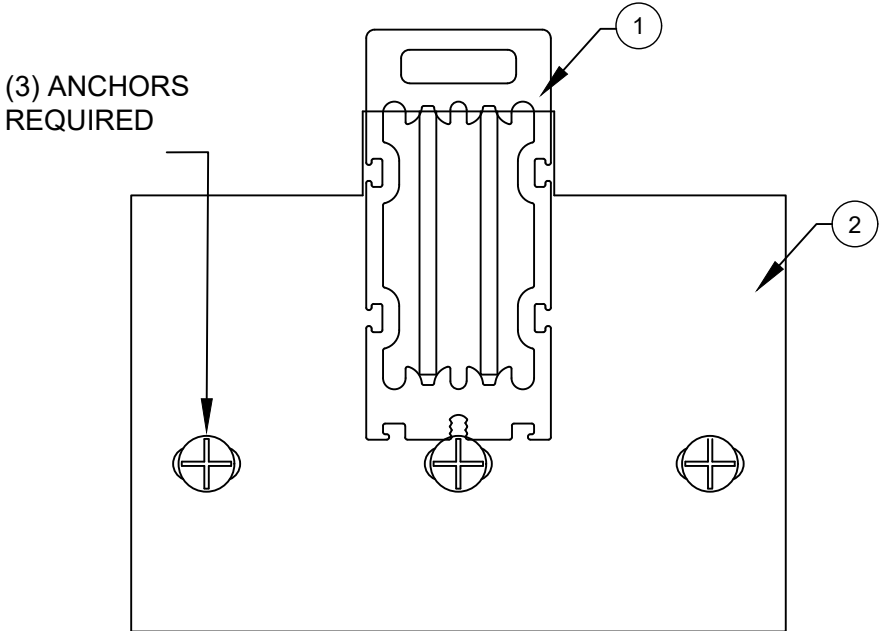
BRACKET (3419) TO MULLION DETAILS (WOOD ANCHOR INSTALLATION)
