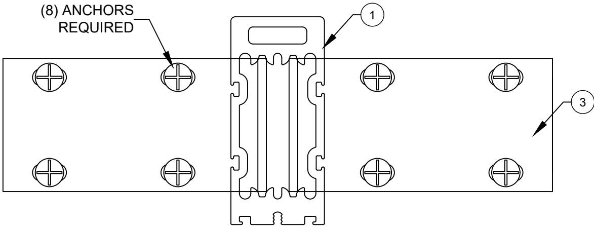
BRACKET (3418) TO MULLION DETAILS (WOOD ANCHOR INSTALLATION)
