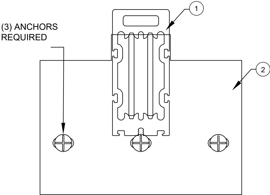
BRACKET (3419) TO MULLION DETAILS (HOLLOW BLOCK OR 3K CONCRETE ANCHOR INSTALLATION)
