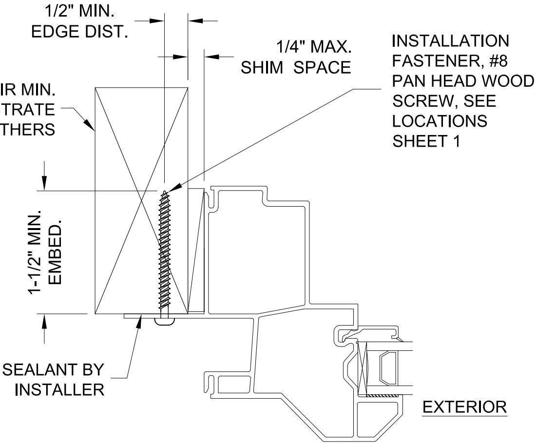
TYPICAL FIN JAMB HORIZONTAL SECTION
