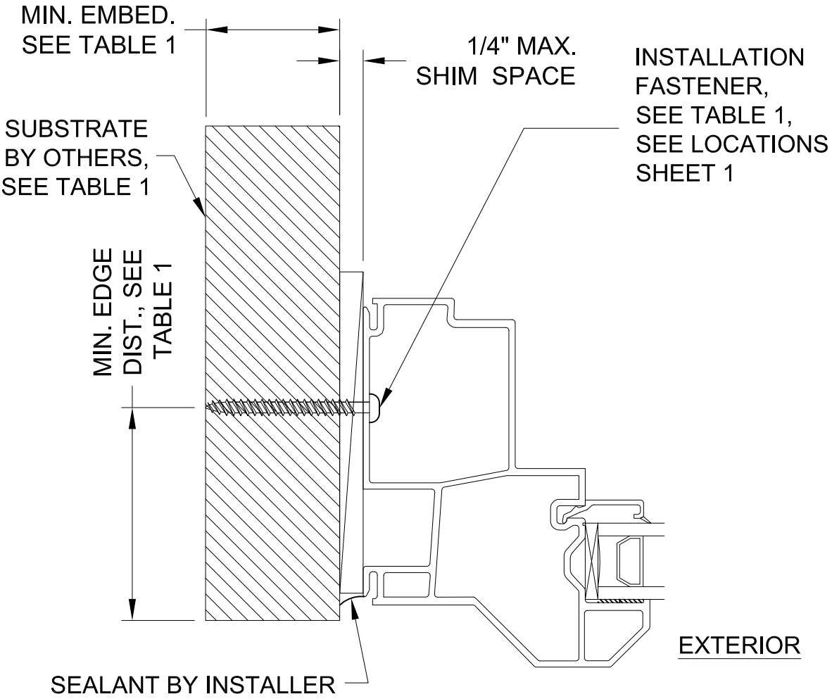
TYPICAL EQUAL LEG JAMB HORIZONTAL SECTION
