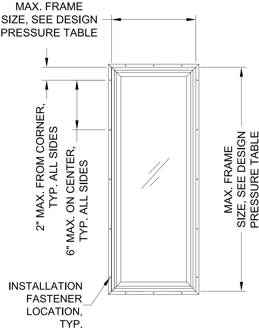
FIN ELEVATION SEE DETAILS SHEETS 3
