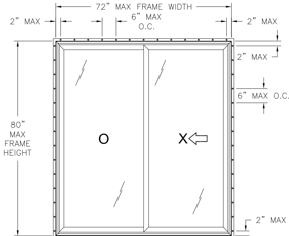
SERIES 1000 HP SLIDING GLASS DOOR EXTERIOR VIEW FIN INSTALLATION
