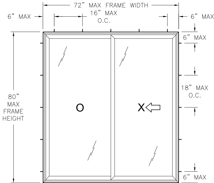
SERIES 1000 HP SLIDING GLASS DOOR EXTERIOR VIEW FRAME INSTALLATION
