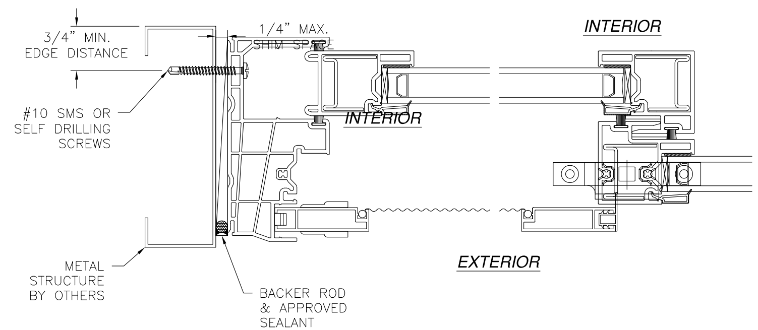
JAMB INSTALLATION DETAIL METAL STRUCTURE INSTALLATION
