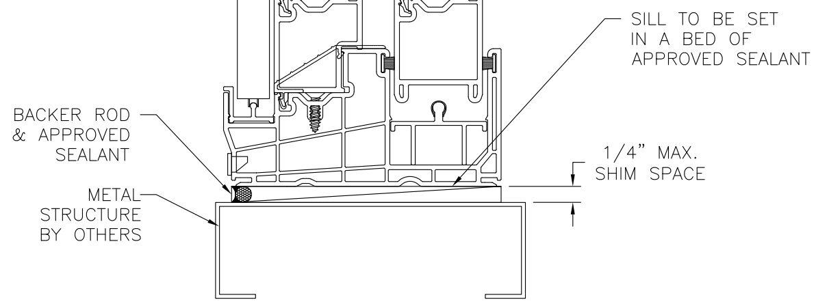
VERTICAL CROSS SECTION METAL STRUCTURE INSTALLATION
