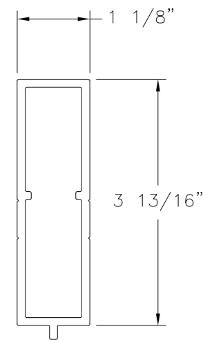
SECT5765 MULLION ALUMINUM 6005-T5 .125" THICK
