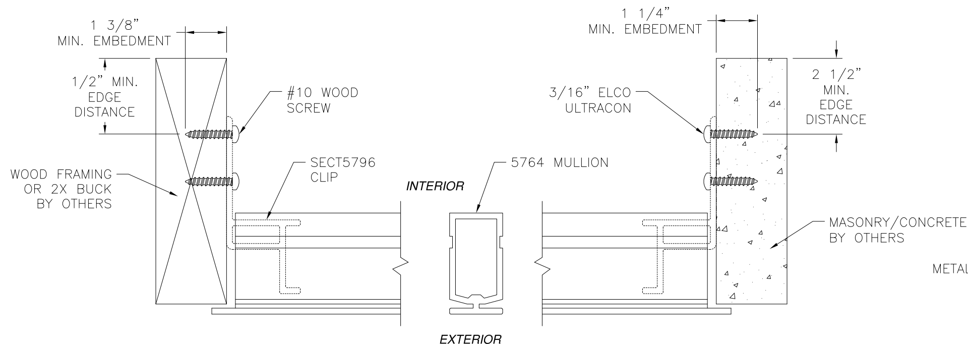
MULLION INSTALLATION WOOD & CONCRETE
