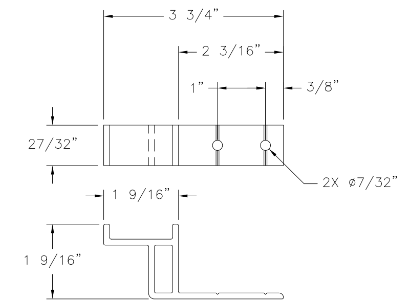
SECT5796 CLIP FOR WOOD FRAMING INSTALLATION ALUMINUM 6063-T5 .125" THICK
