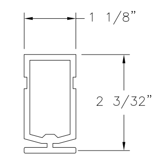
SECT5764 MULLION ALUMINUM 6005-T5 .125" THICK
